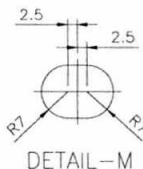
DETAIL-M
