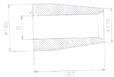
1. LADLE NOZZLE
