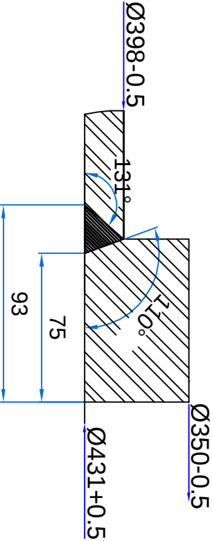
DETAIL A
