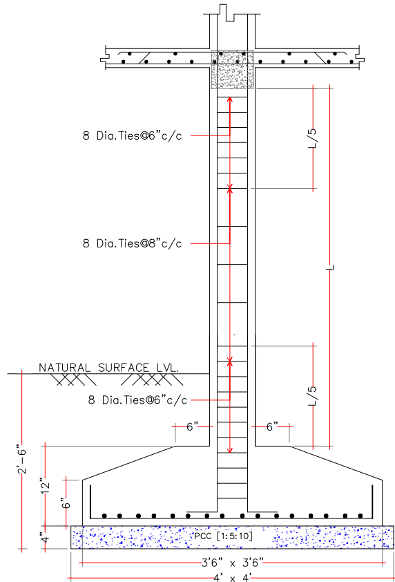
GUIDE SECTION THROUGH FOOTING
