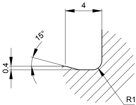
DETAIL - X
