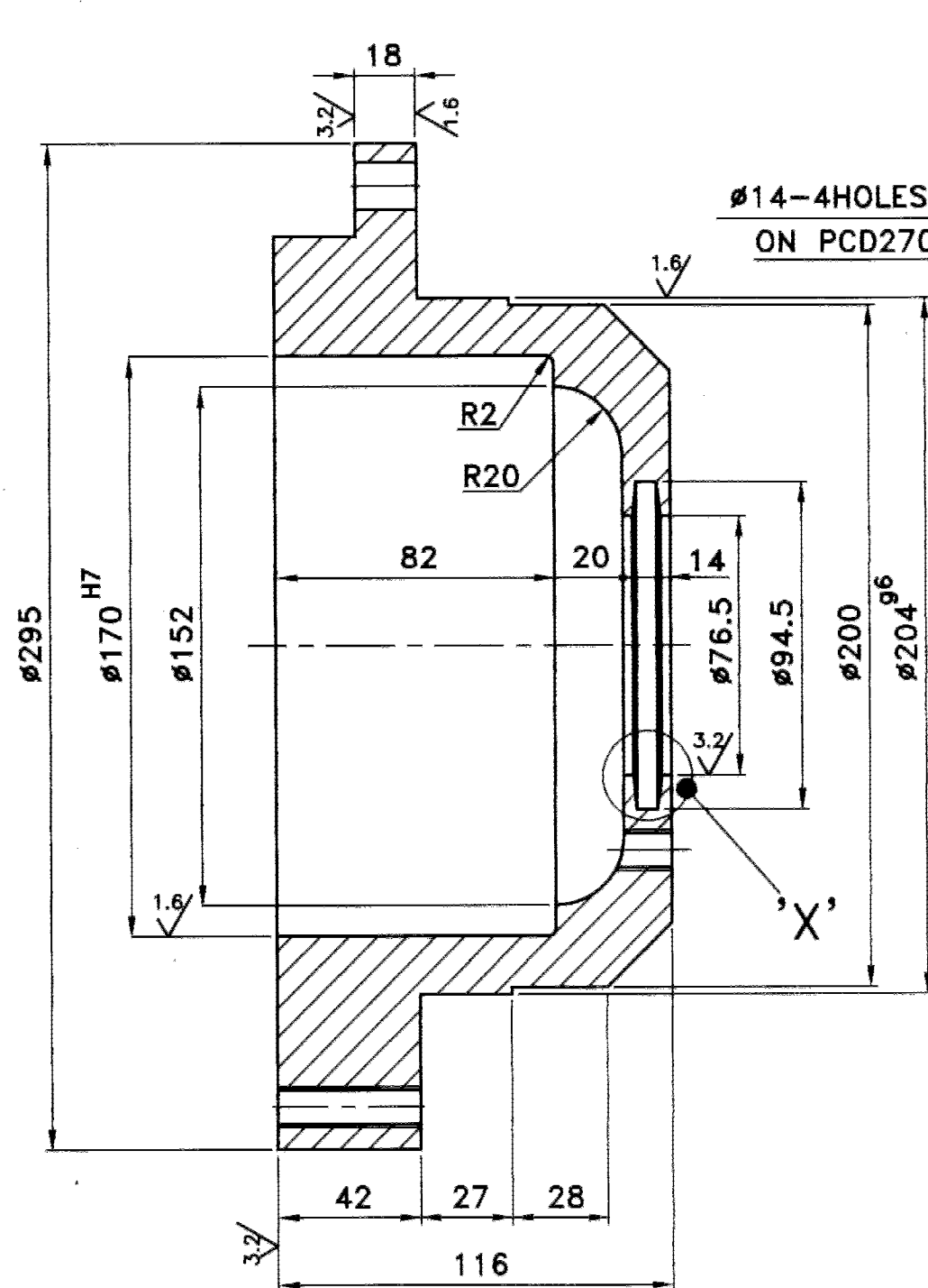
SECTION-AA
