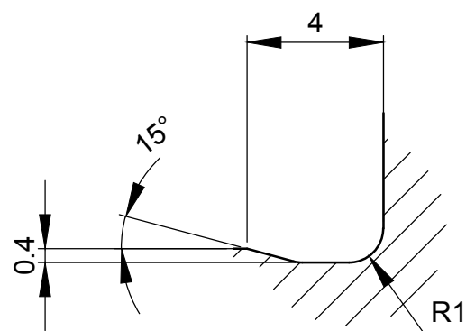
DETAIL - X
