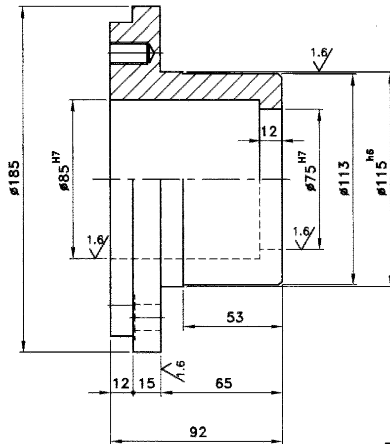
SECTION-AA
