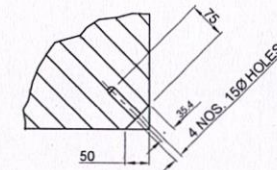
DETAIL -Y
