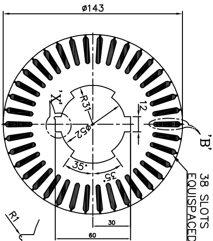
SECTION-'Y'
