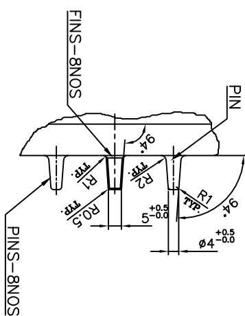
DETAIL-'Z'
