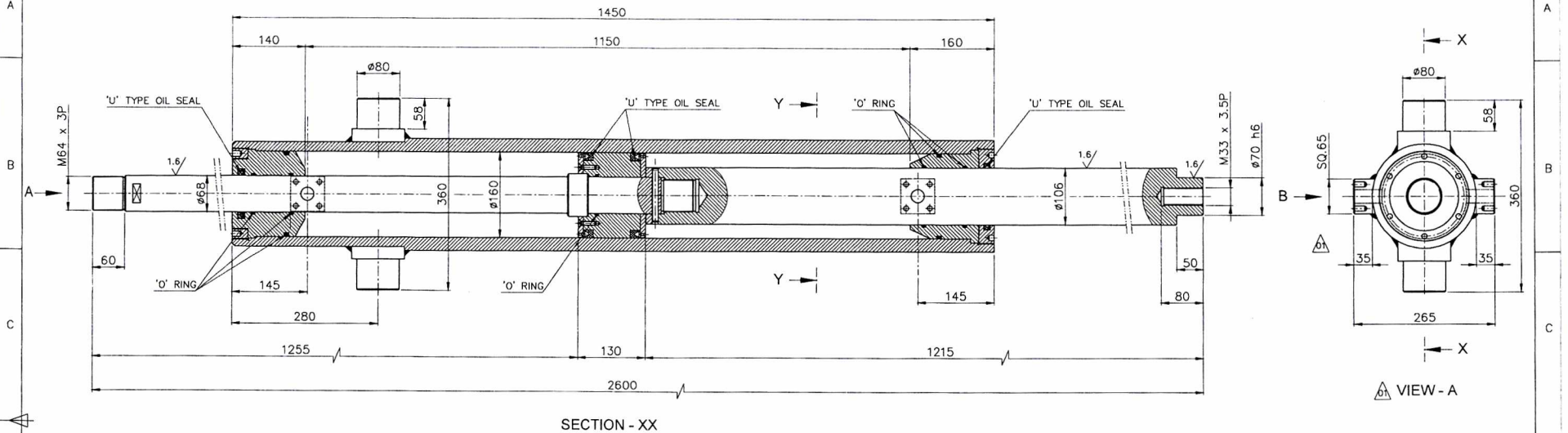
SECTION - XX
