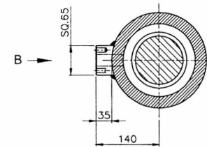
SECTION - YY
