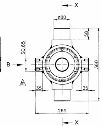
VIEW - A
