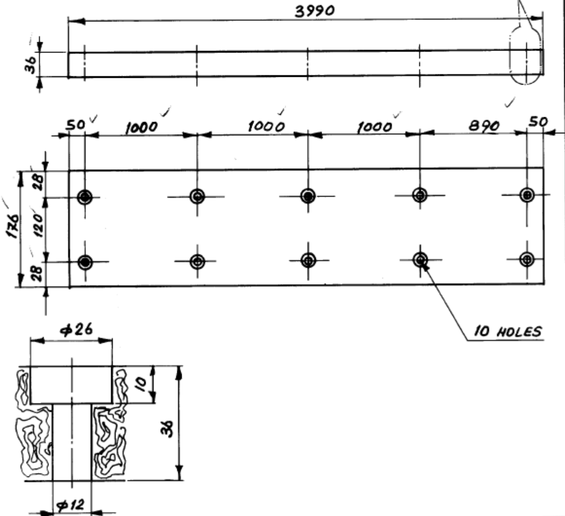
DETAIL - X
