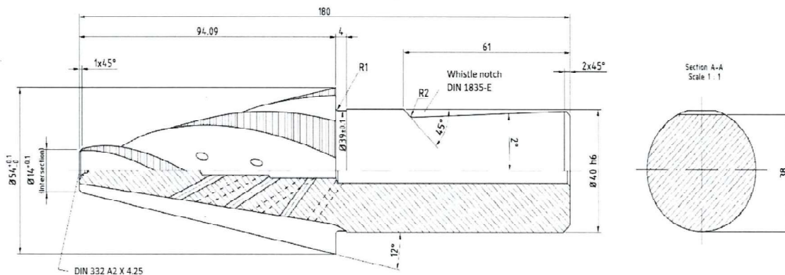
SKETCH -C (Drawing of Conical cutter FORM 17)
