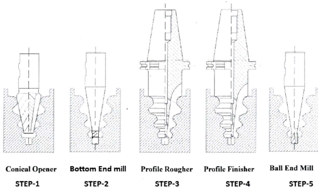
SKETCH SHOWING SCHEMATIC DRAWING OF FIRTREE GROOVE MACHINING
