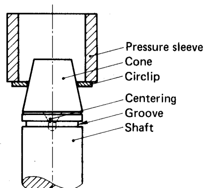
Figure 14. Fitting with cones
