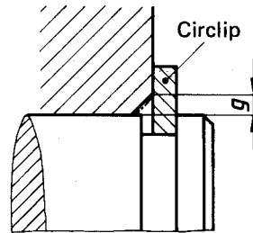
Figure 8. Abutment with edge chamfering distance (chamfering or rounding)
