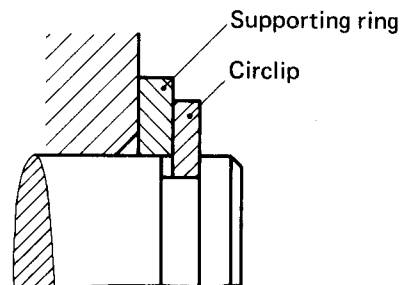
Figure 9. Sharp-edged abutment at the circlip using a supporting ring
