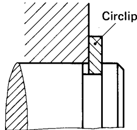
Figure 7. Sharp-edged abutment
