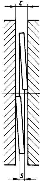
Figure 6. Testing the spiral flatness
