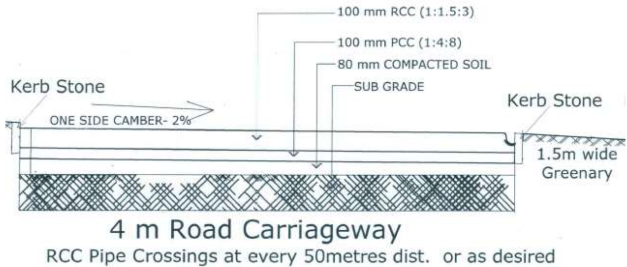
Cross Sectional Details Admin Area Connecting Road (Package B)
