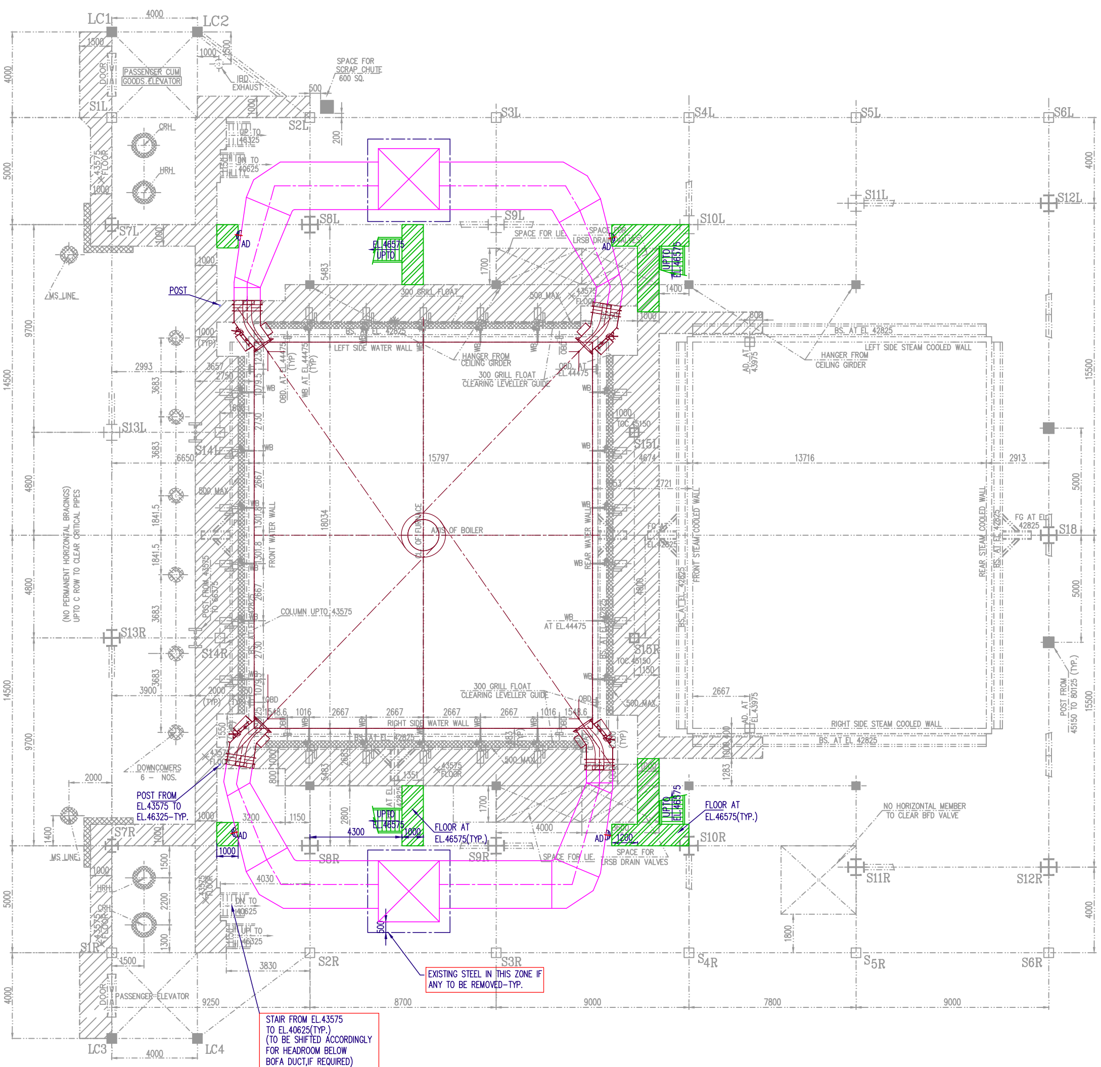
FLOOR PLAN AT EL.43575 (MBL-4)
