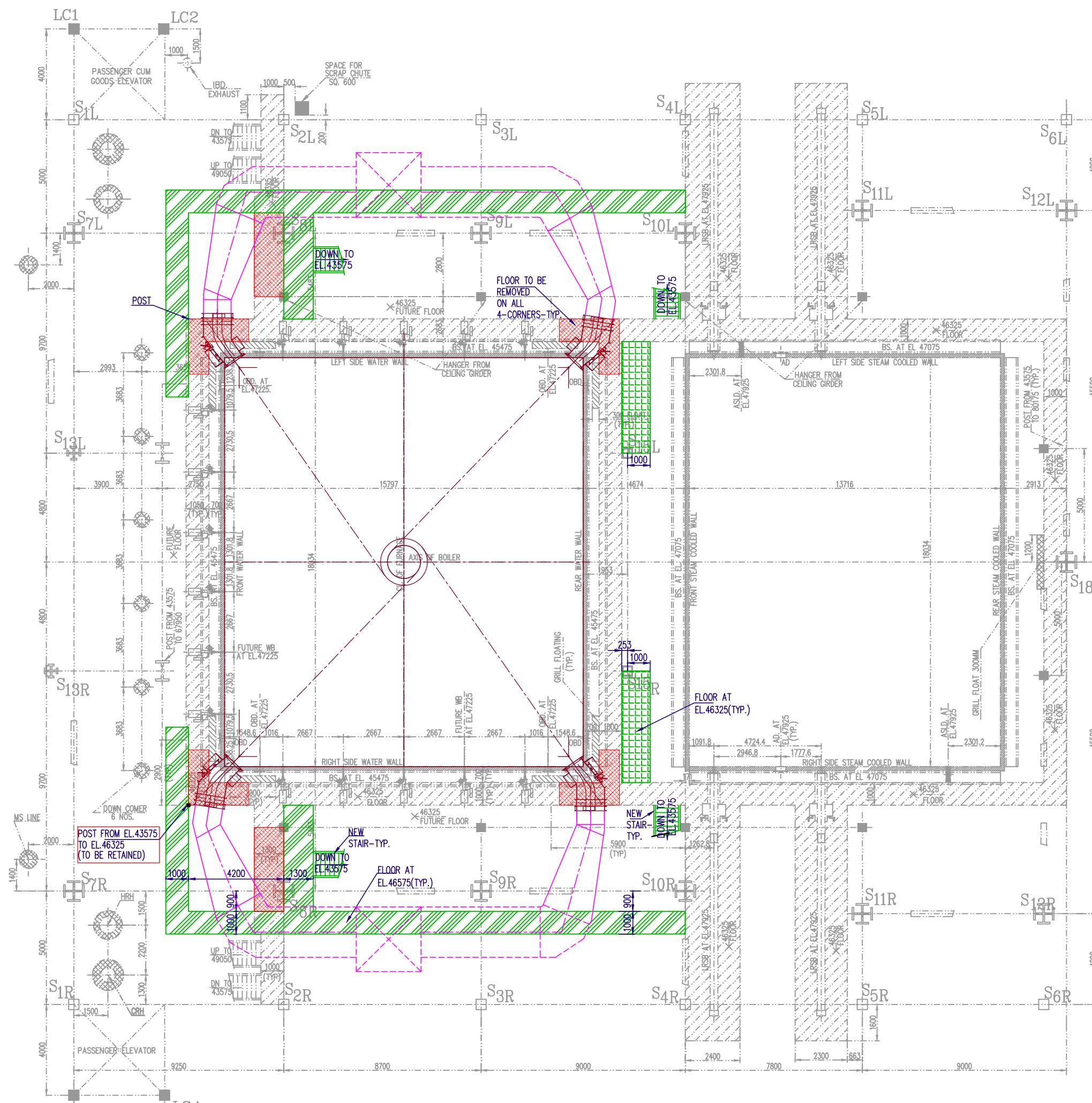
FLOOR PLAN AT EL.46325
