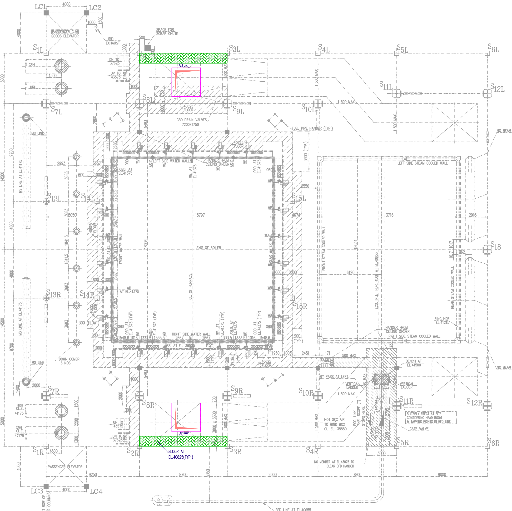
FLOOR PLAN AT EL.40625
