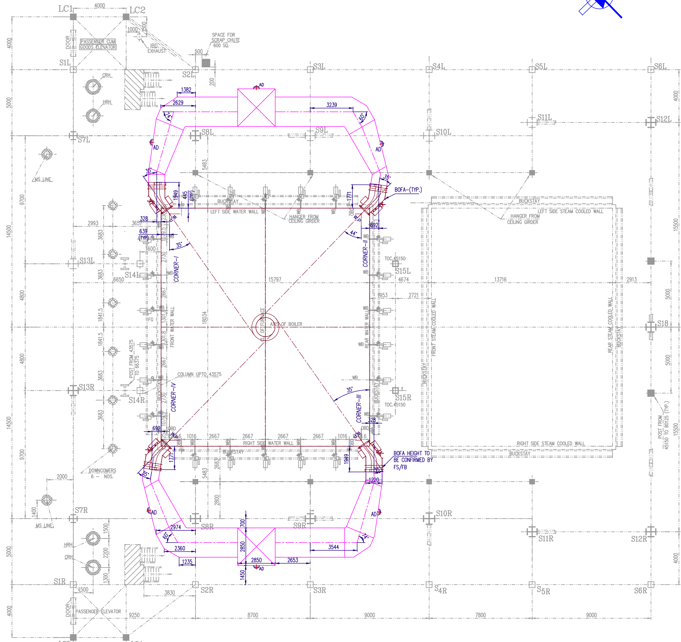
PLAN VIEW
