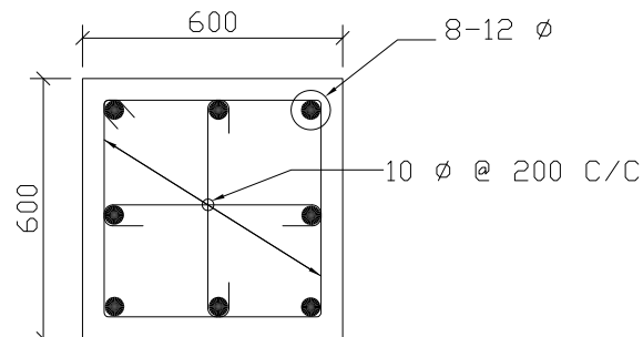
SECTION 4-4
