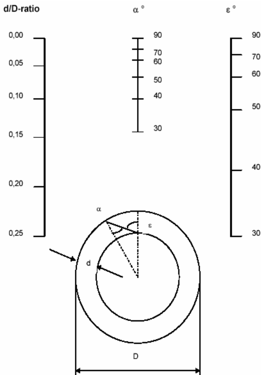
Figure 1: Diagram for Determination of Incidence Angle \varepsilon as Function of curvature Geometry for Evidence of Cracks at the Opposite Surface
