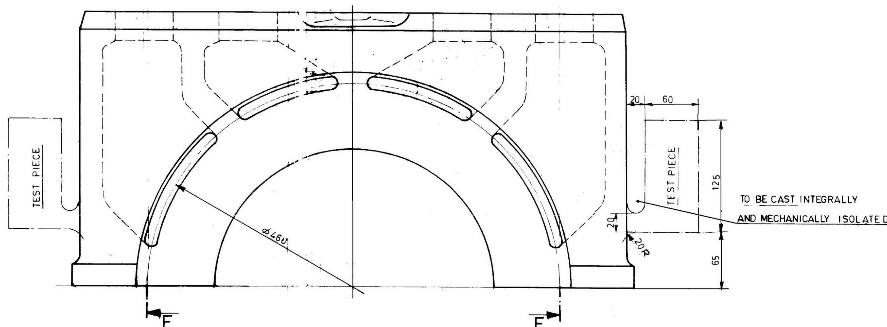
VIEW-H
