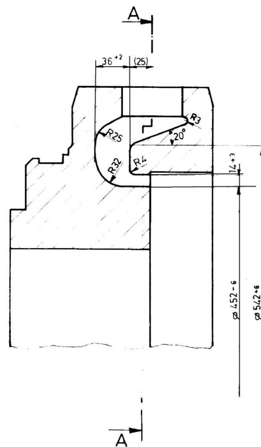
SECTION C-C
