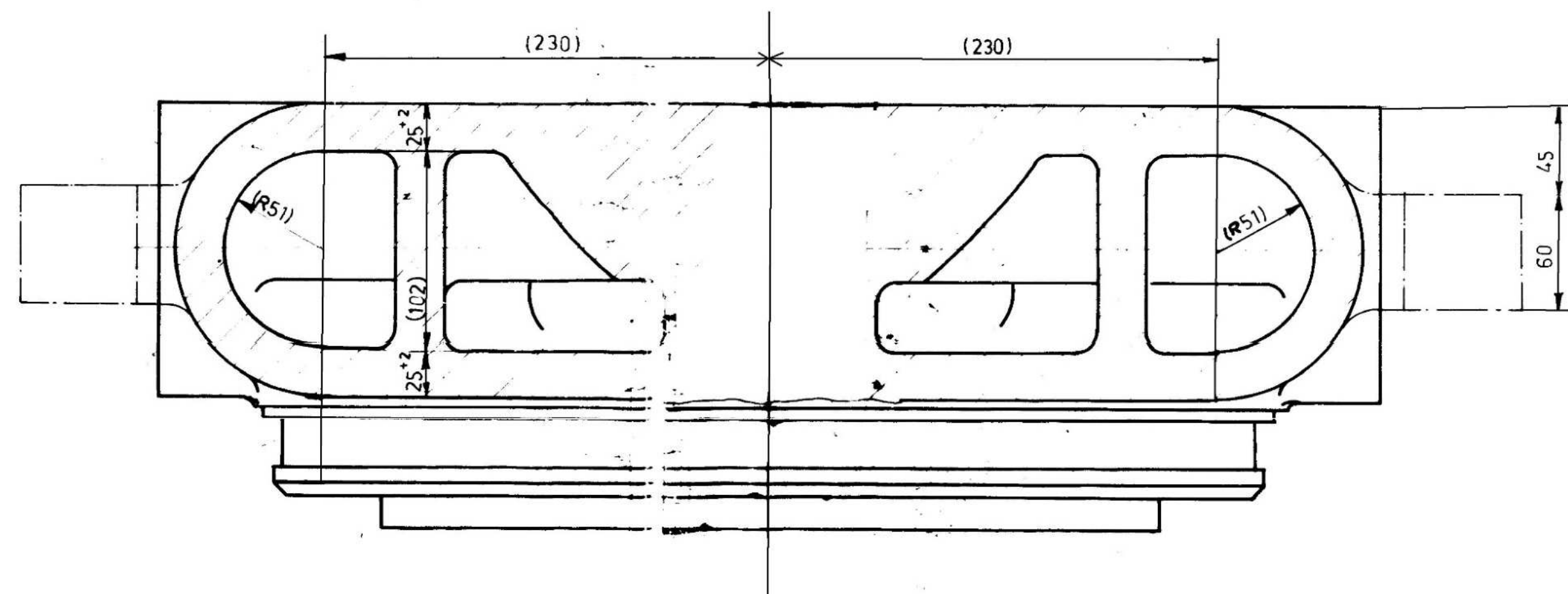
SECTION E-E
