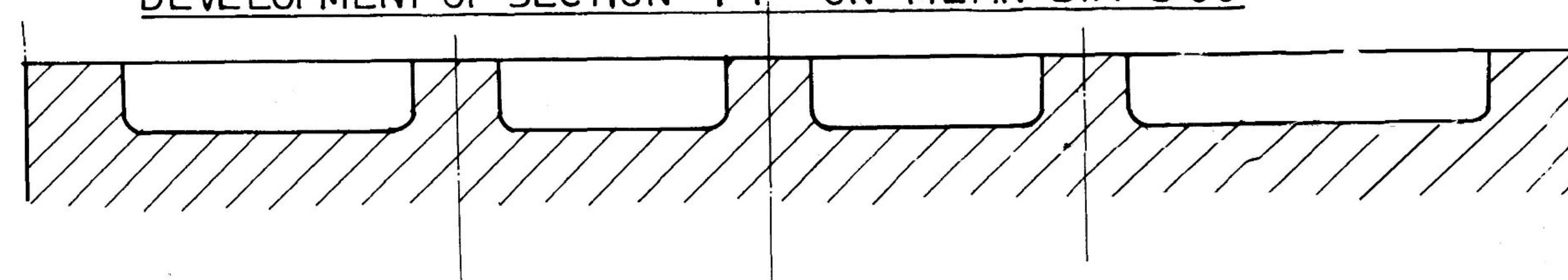
DEVELOPMENT OF SECTION F-F ON MEAN DIA. 900
