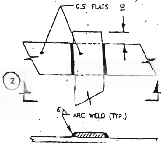
SECTION - ②
