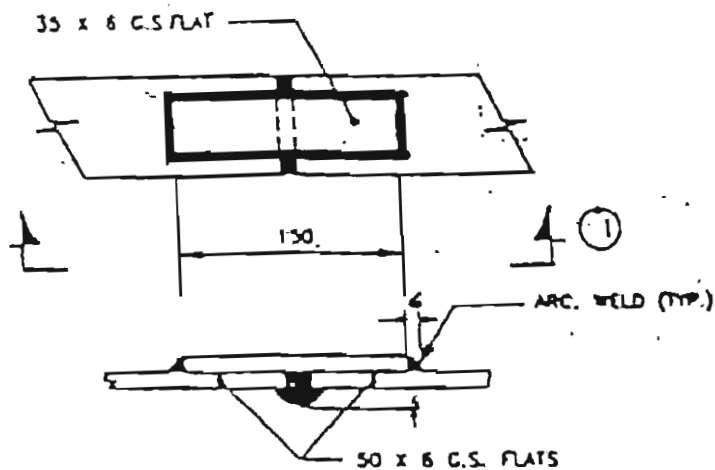
SECTION - ①
