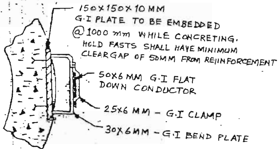
DETAIL- "Y"
