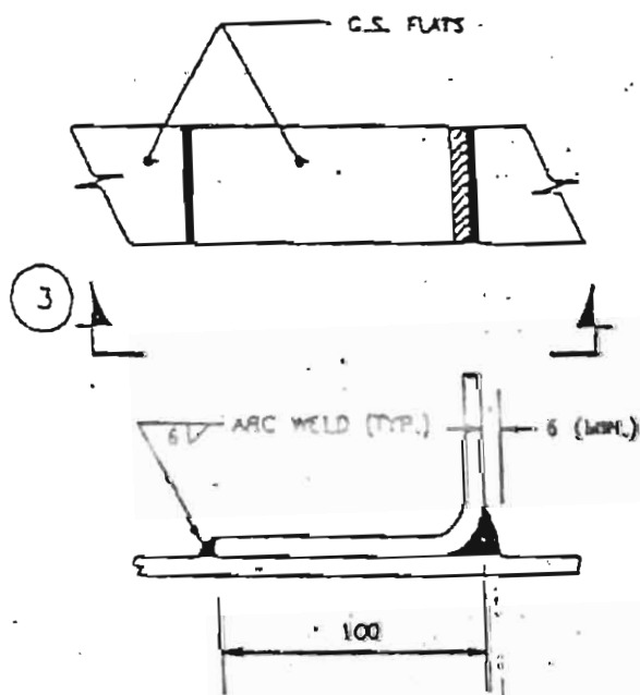
SECTION - ③
