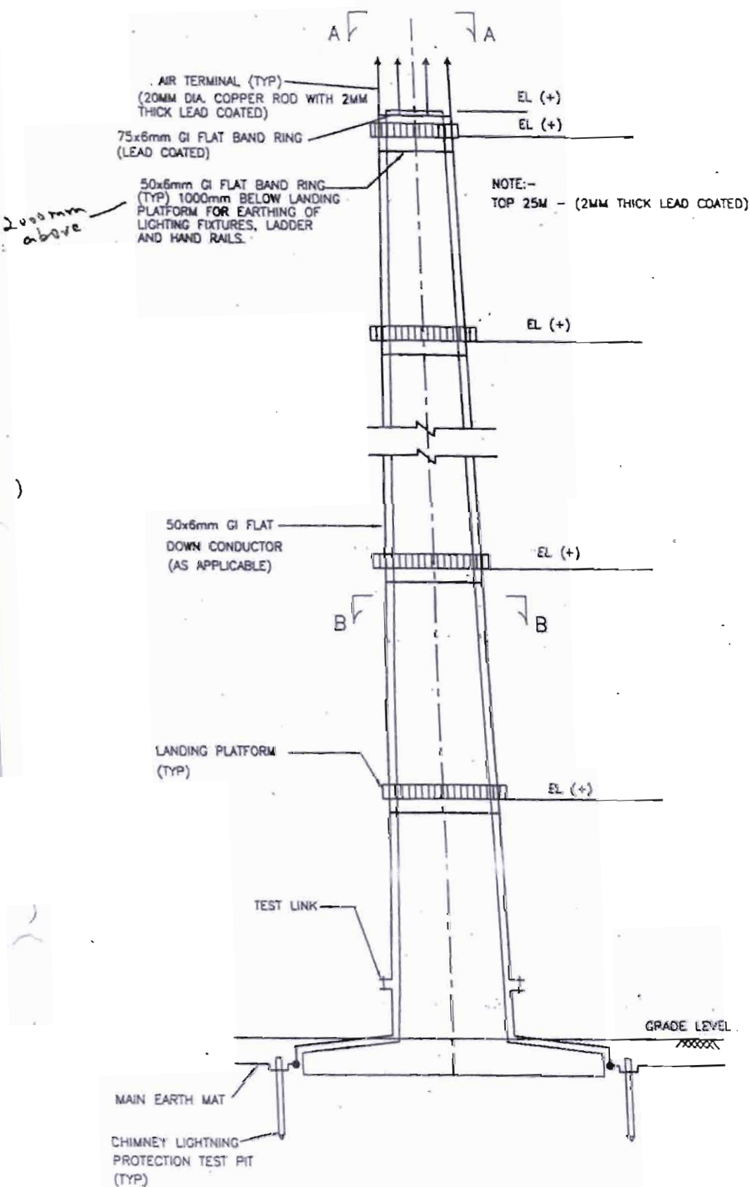
CHIMNEY (ELEVATION)
