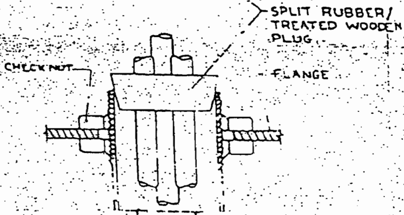
CLAMPING OF WIRES IN CONDUIT VERTICAL RUN
