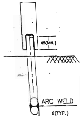
SECTION 3-3
