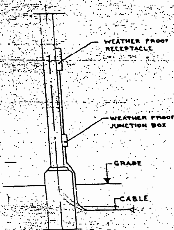
OUTDOOR RECEPTACLE
