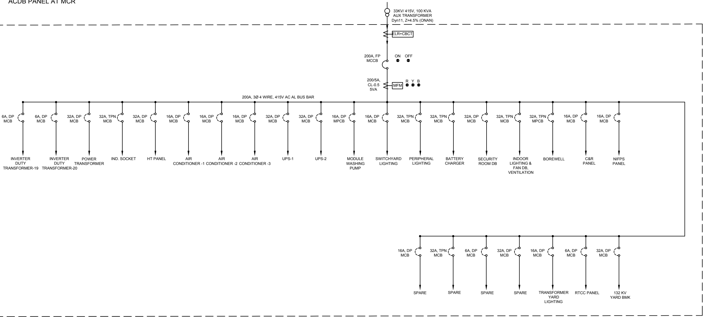
AC AUXILIARY POWER SUPPLY SCHEME IN MCR
