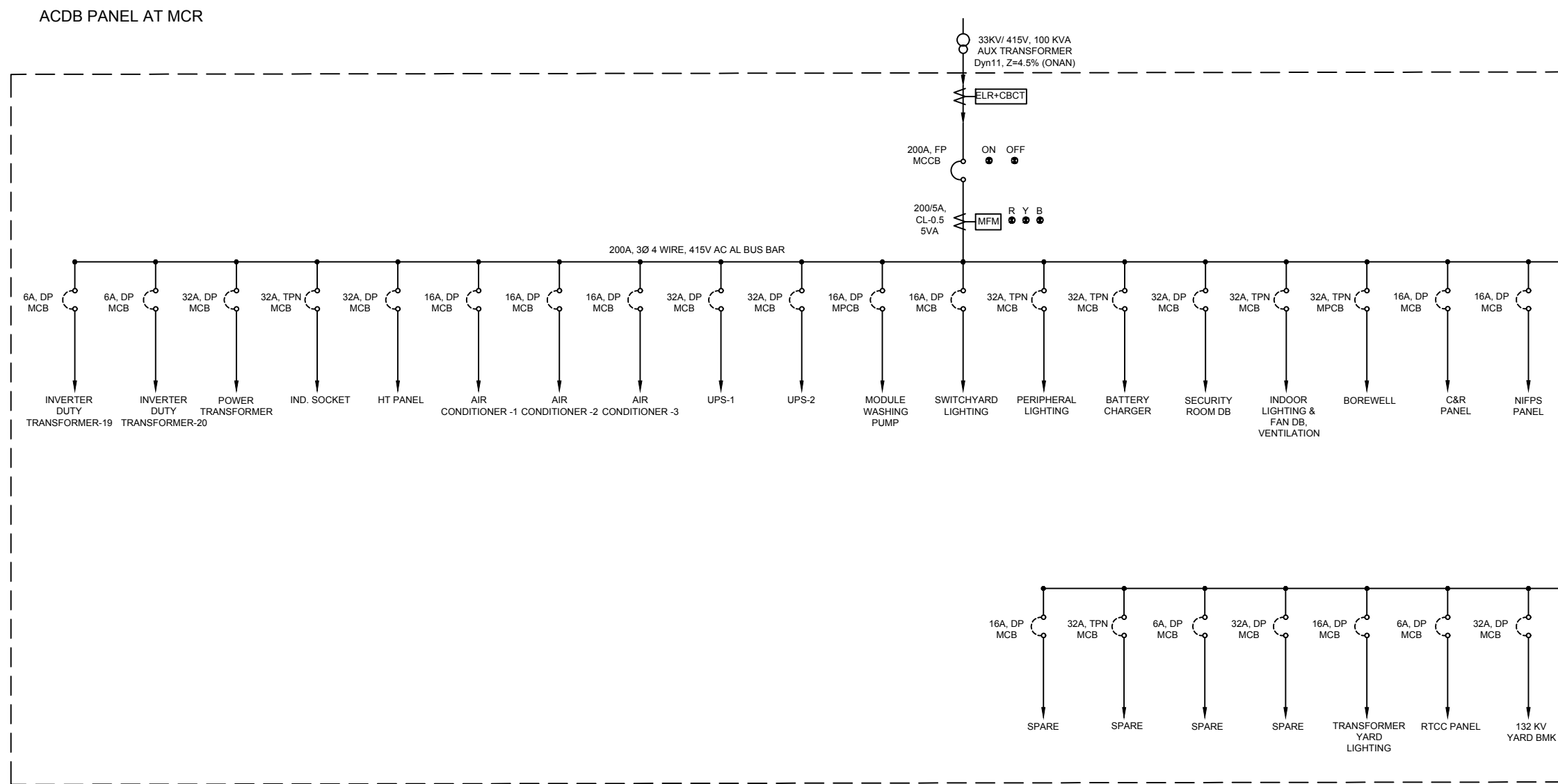
AC AUXILIARY POWER SUPPLY SCHEME IN MCR
