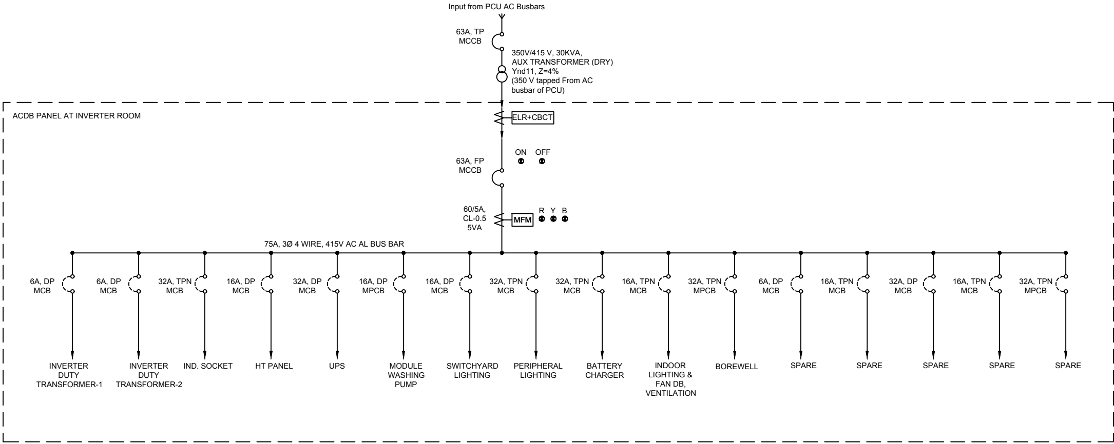
AC AUXILIARY POWER SUPPLY SCHEME IN ICR
