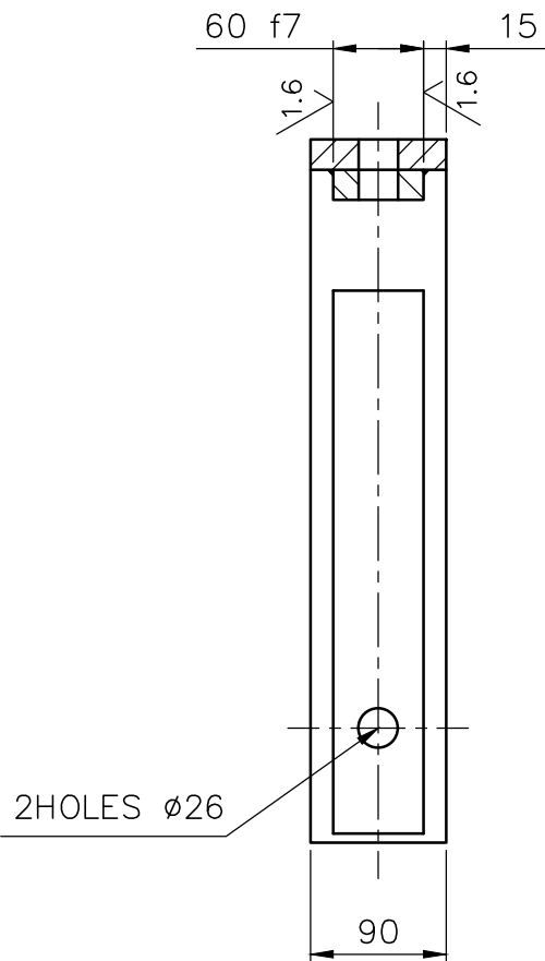
SECTION - AA
