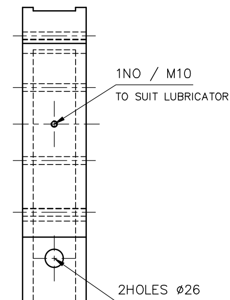
VIEW -B
