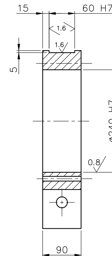
SECTION - AA
