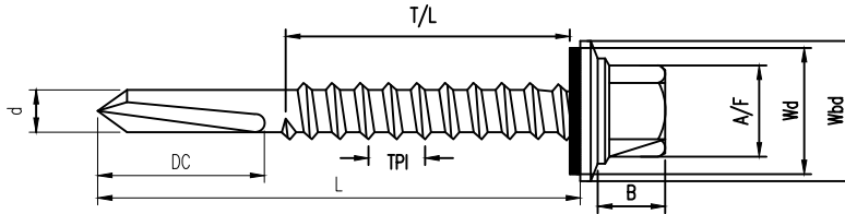
TYPICAL SCREW DETAIL
