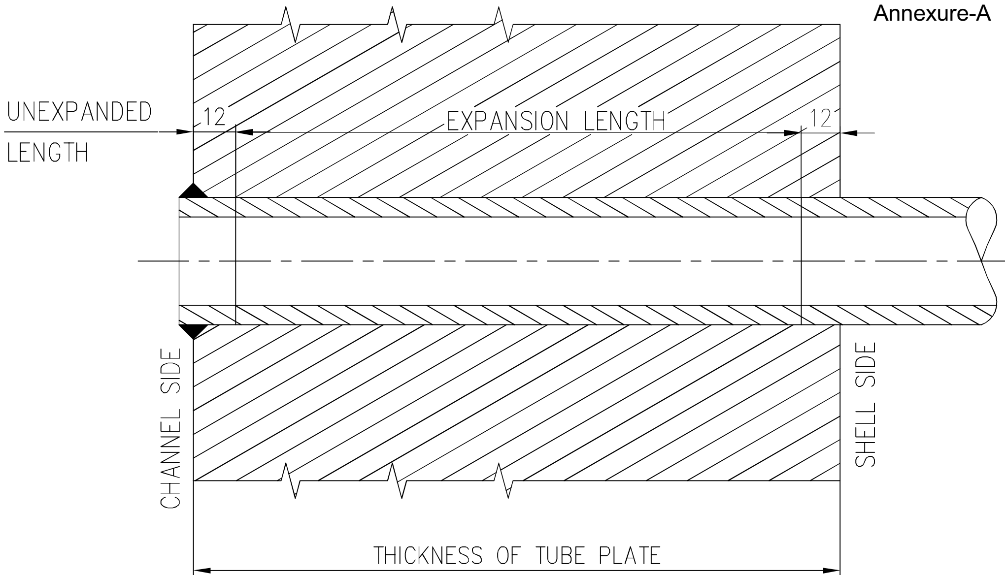
EXPANSION DETAIL
