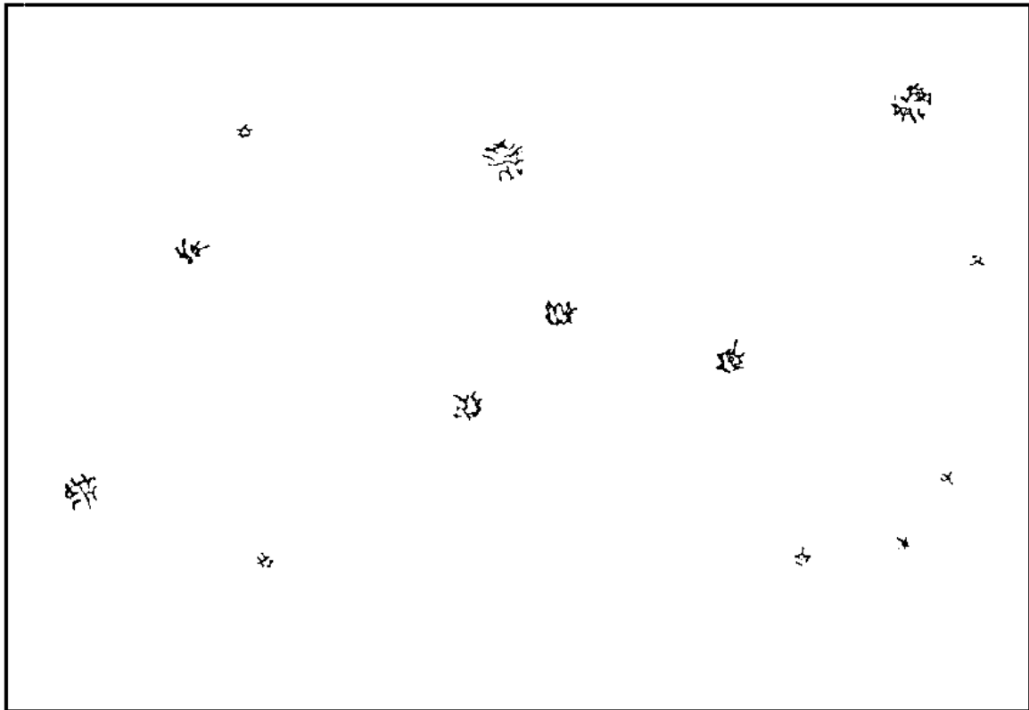
Fig. 7: Grade 3 – magnetic particle testing
