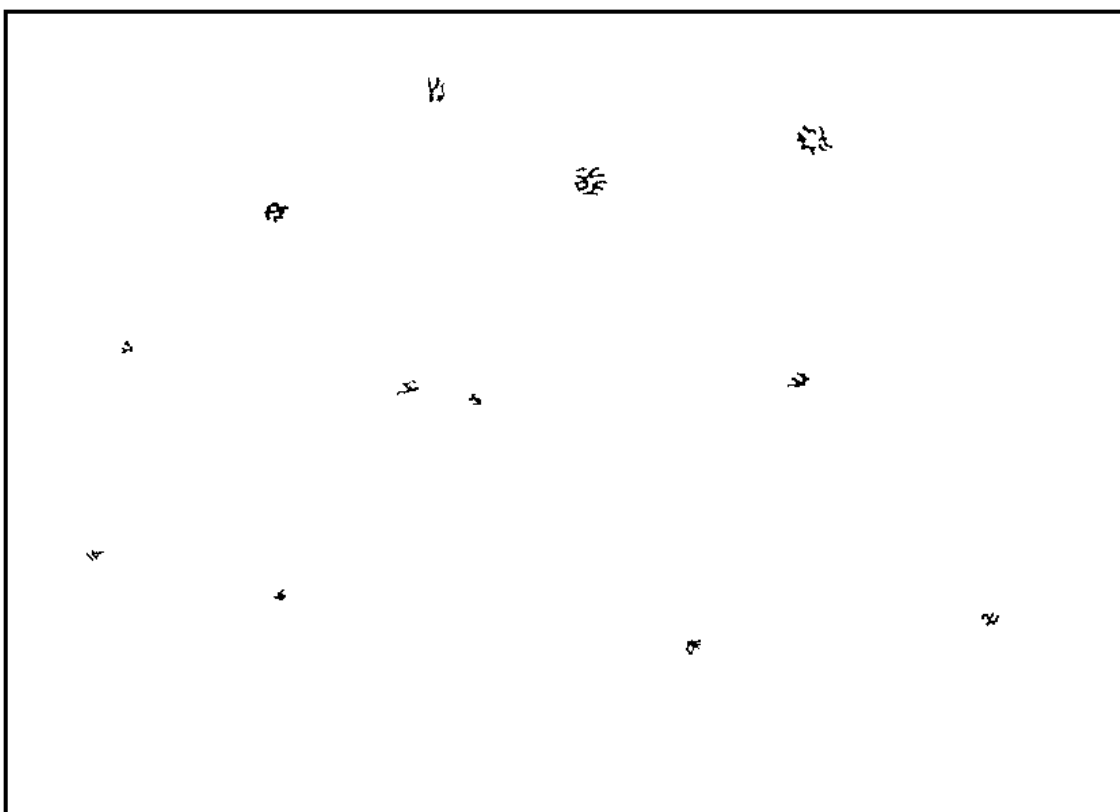
Fig. 6: Grade 2 – magnetic particle testing
