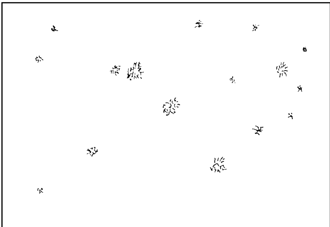
Fig. 8: Grade 4 – magnetic particle testing
