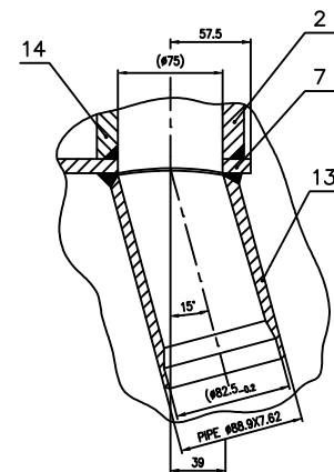
SECTION-BB SCALE:-1:2
