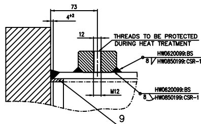
VIEW-A
