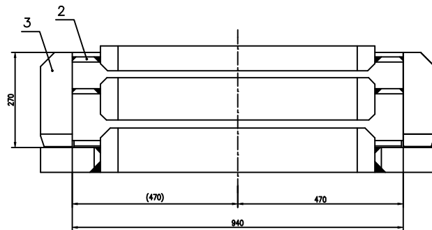
VIEW ON THE JOINT PLANE OF UPPER HALF
