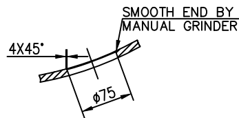
VIEW-Z SCALE-1:5
