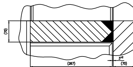
SECTION-CC SCALE:-1:2.5
