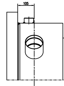
VIEW-W
