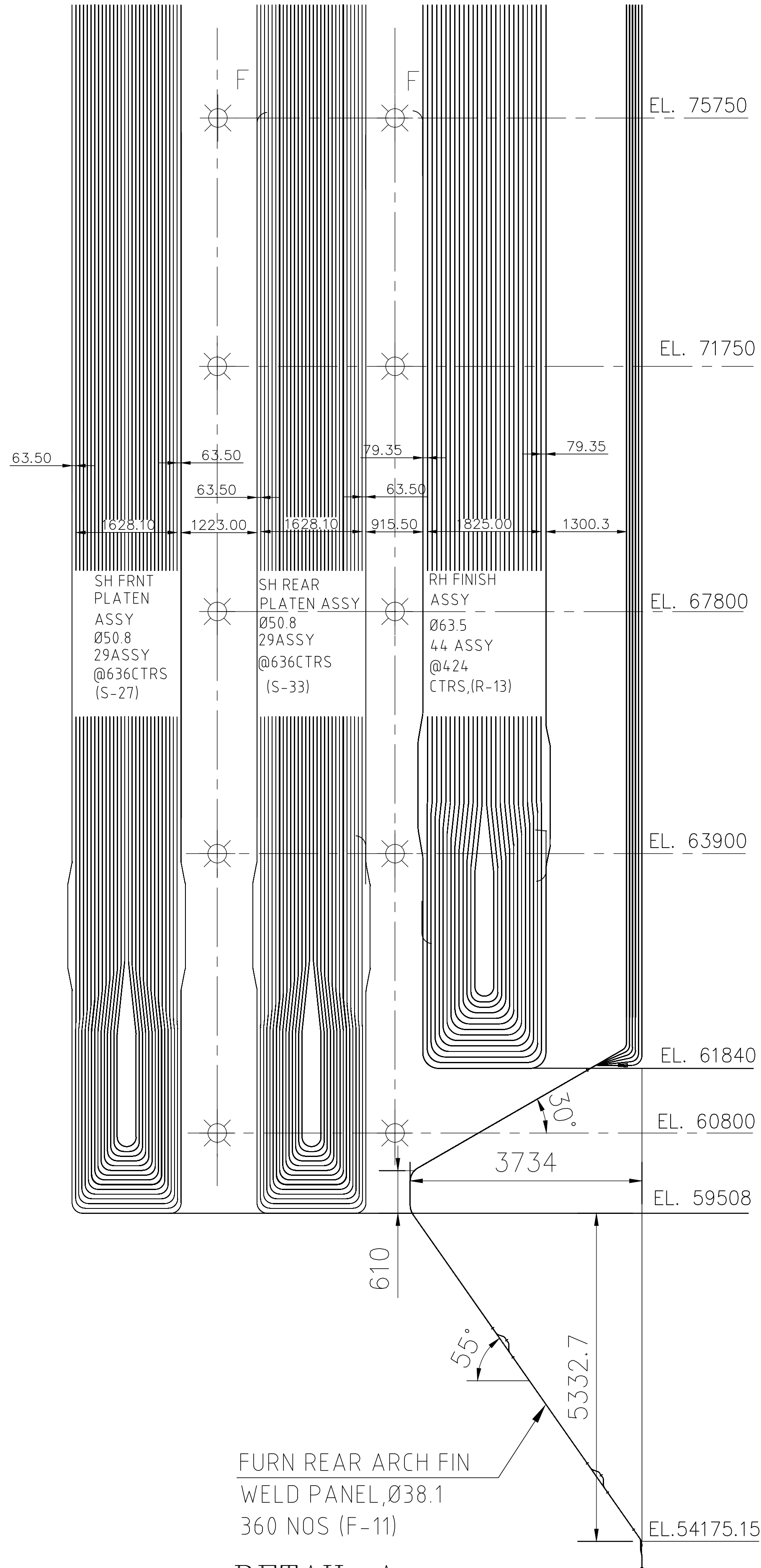
DETAIL A SCALE 1:50
