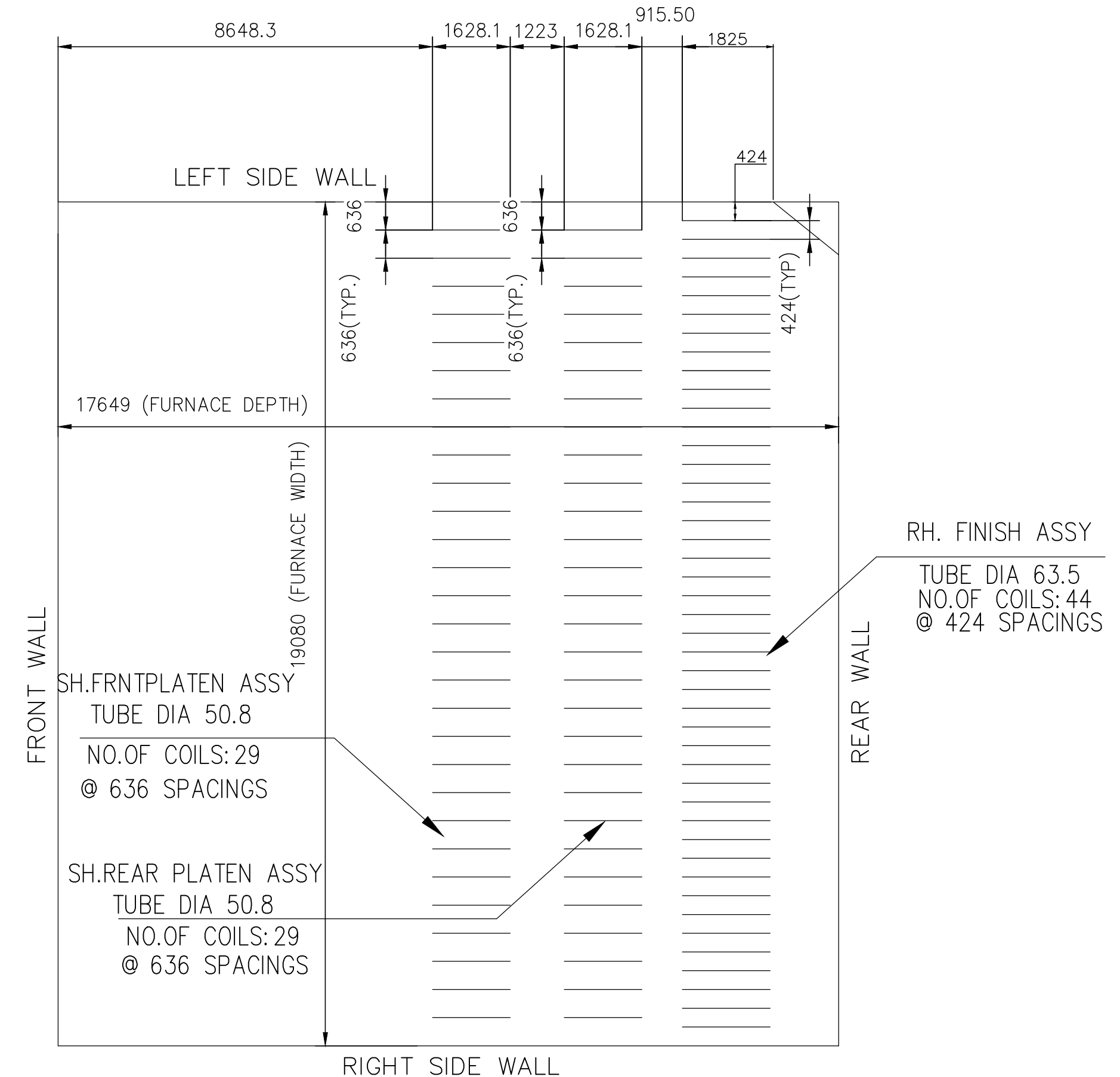
VIEW BB(COIL LEVEL) SCALE 1:100
