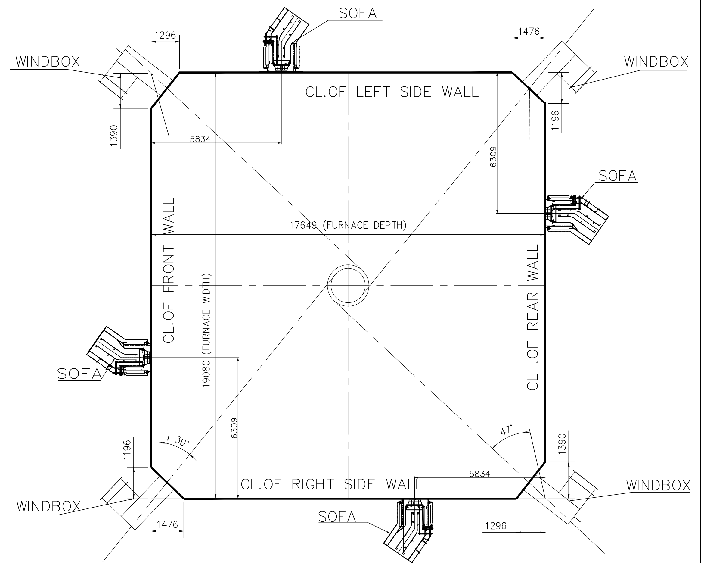
PLAN VIEW("AA" BURNER LEVEL WITH CUT CORNER) SCALE 1:100
