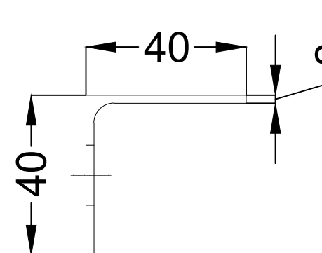
BR1A-BRACING (40LU40x2) SCALE - 20:1
