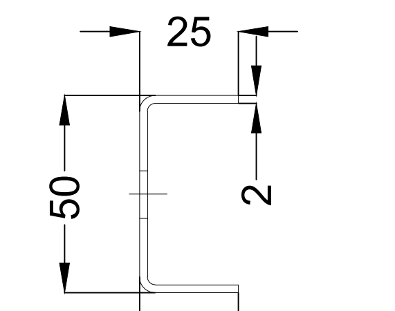
BR1 BRACING (50CU25X2) SCALE - 20:1
