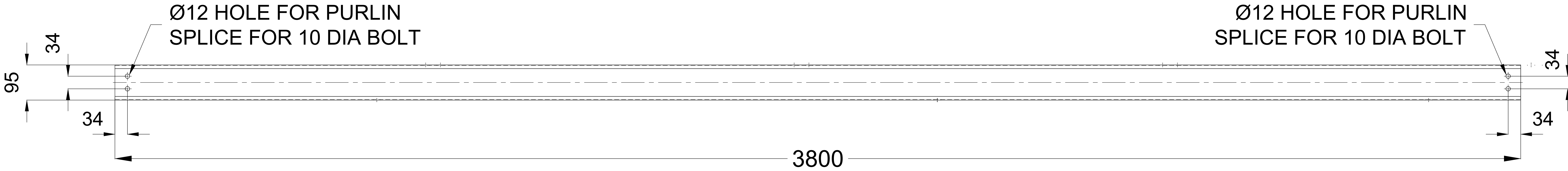
FRONT VIEW
