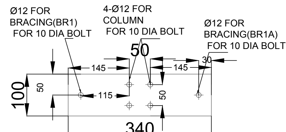
PL2-COLUMN PLATE (340 X100) SCALE - 20:1
