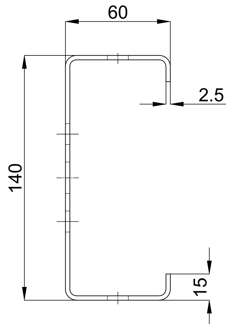
CL1-COLUMN (CS140x60x2.5x15) SCALE - 20:1
