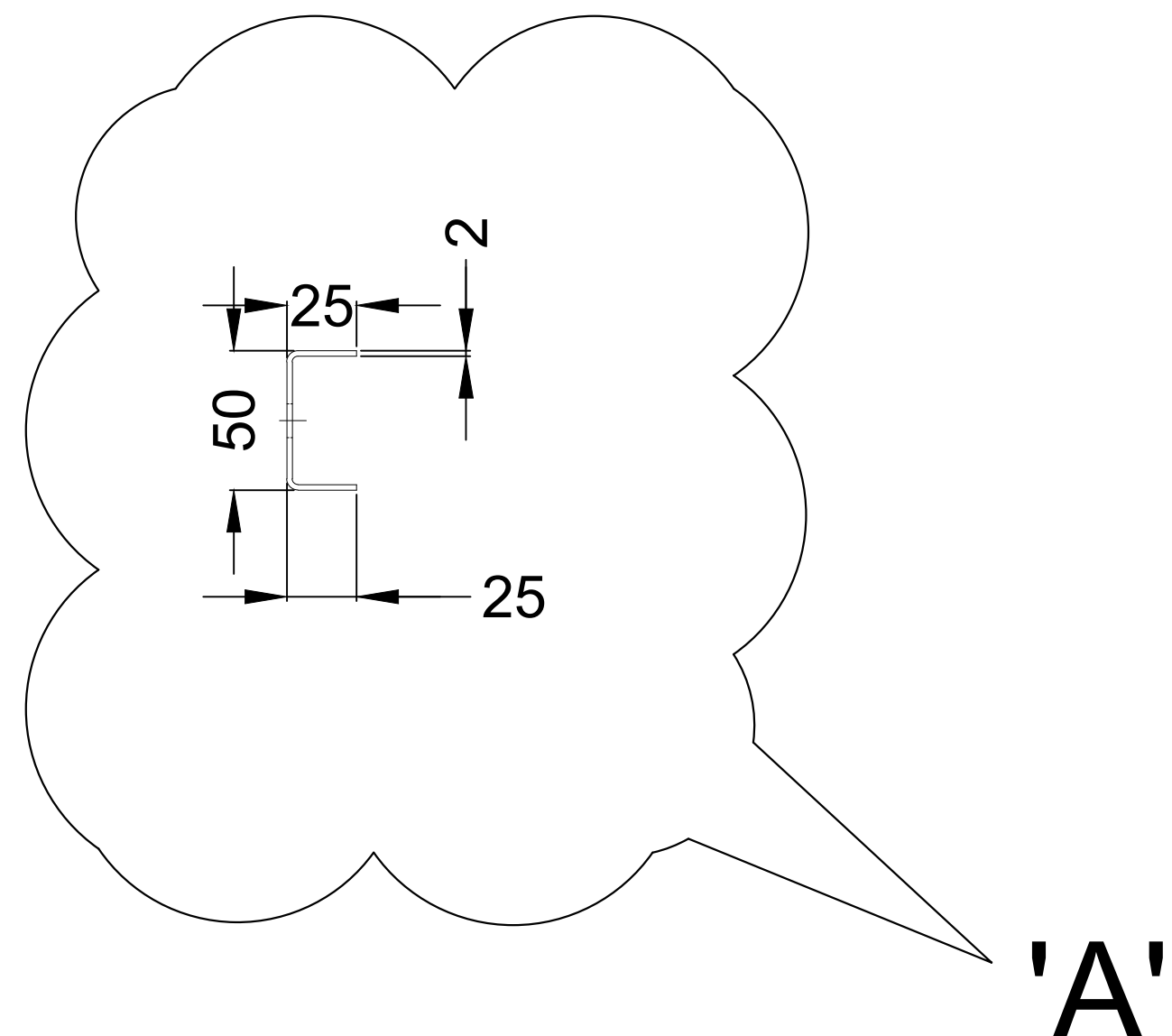
SIDE VIEW
