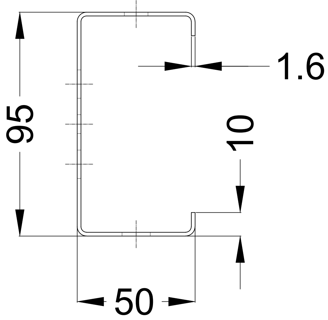
DETAIL – 'A'
