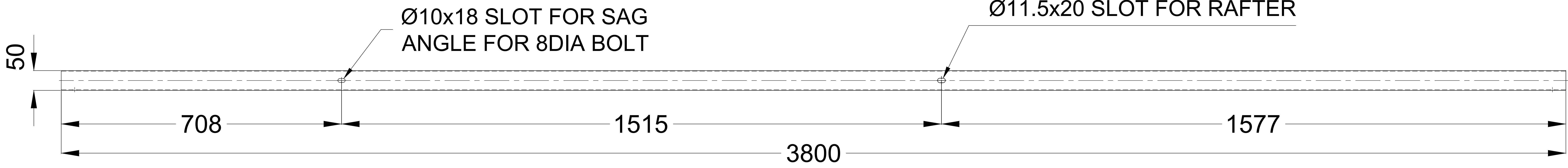
BOTTOM VIEW
