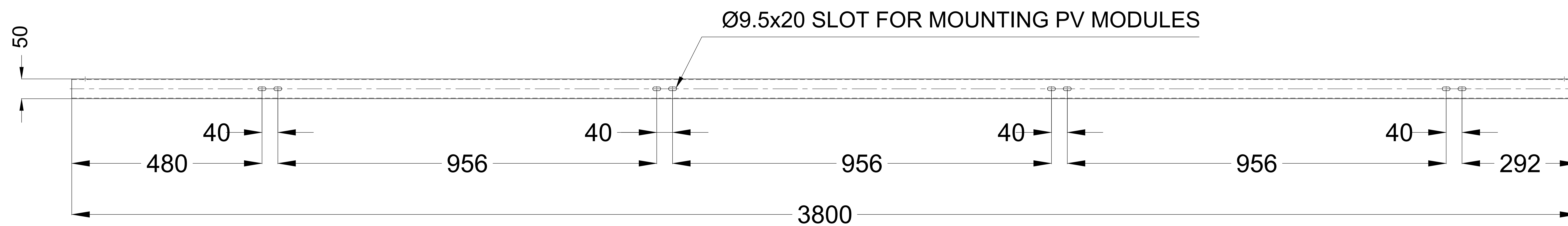
TOP VIEW
