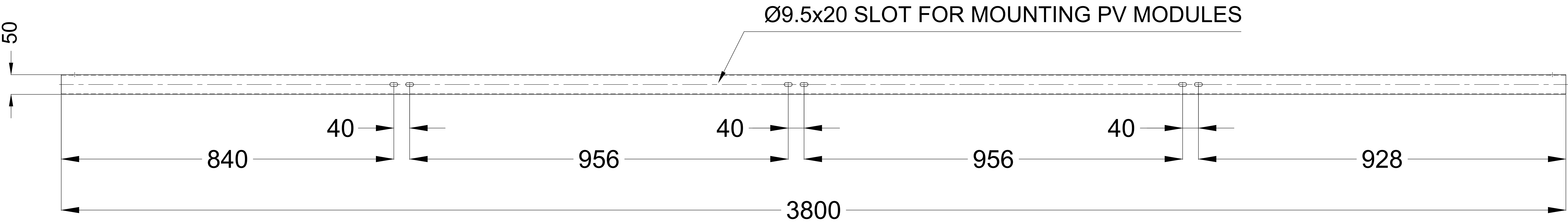
TOP VIEW
