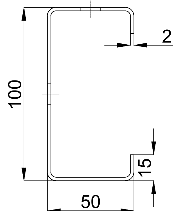
RF1-RAFTER (CS100x50x2x15) SCALE - 20:1
