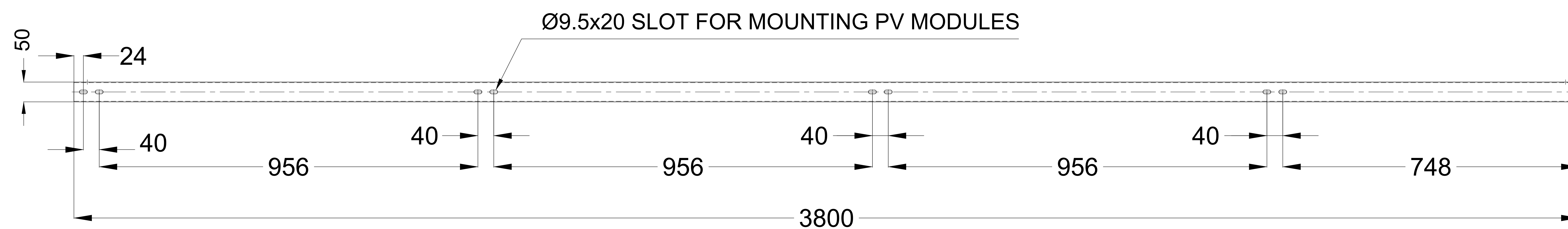
TOP VIEW
