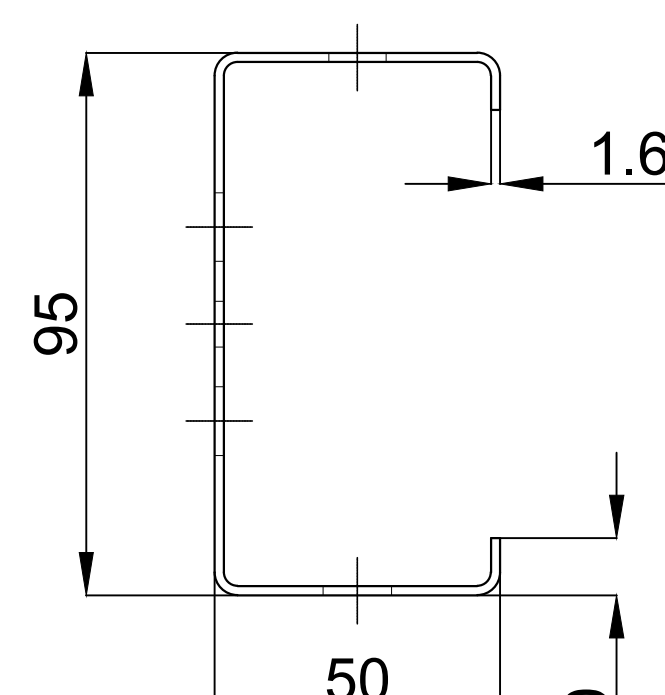
PU-PURLIN (CS95x50x1.6x10) SCALE - 20:1
