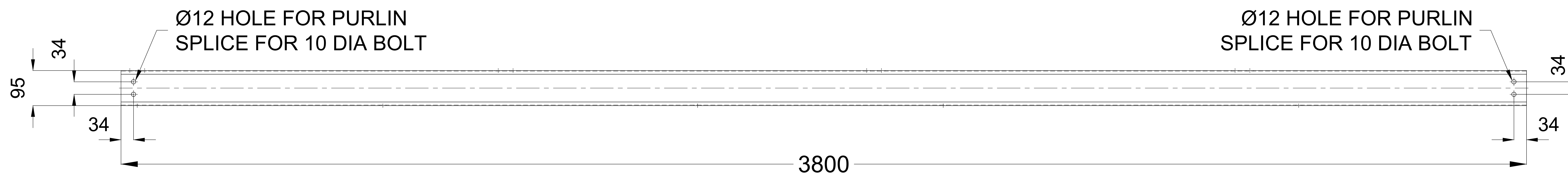
FRONT VIEW
