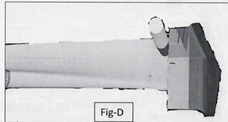
Shroud side fillet after finish operation with tapered Ball nose Cutter (K-6)
