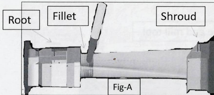
Root side fillet start of operation with tapered Ball nose Cutter(K-6)
