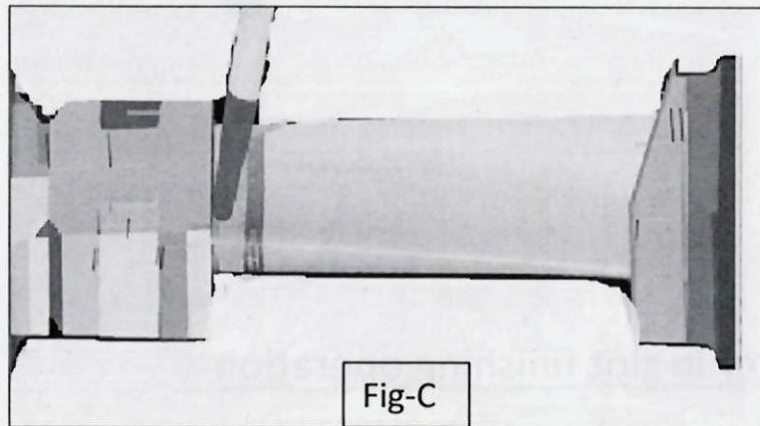
Root side fillet after finish operation with tapered Ball nose Cutter (K-6)
