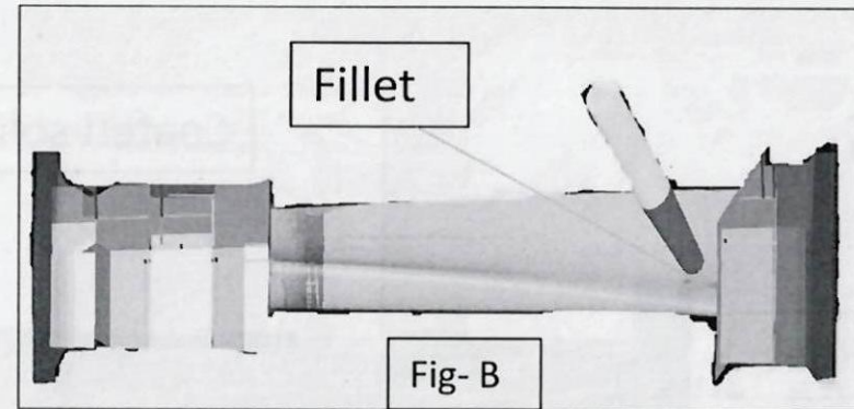
Shroud side fillet start of operation with tapered Ball nose Cutter (K-6)
