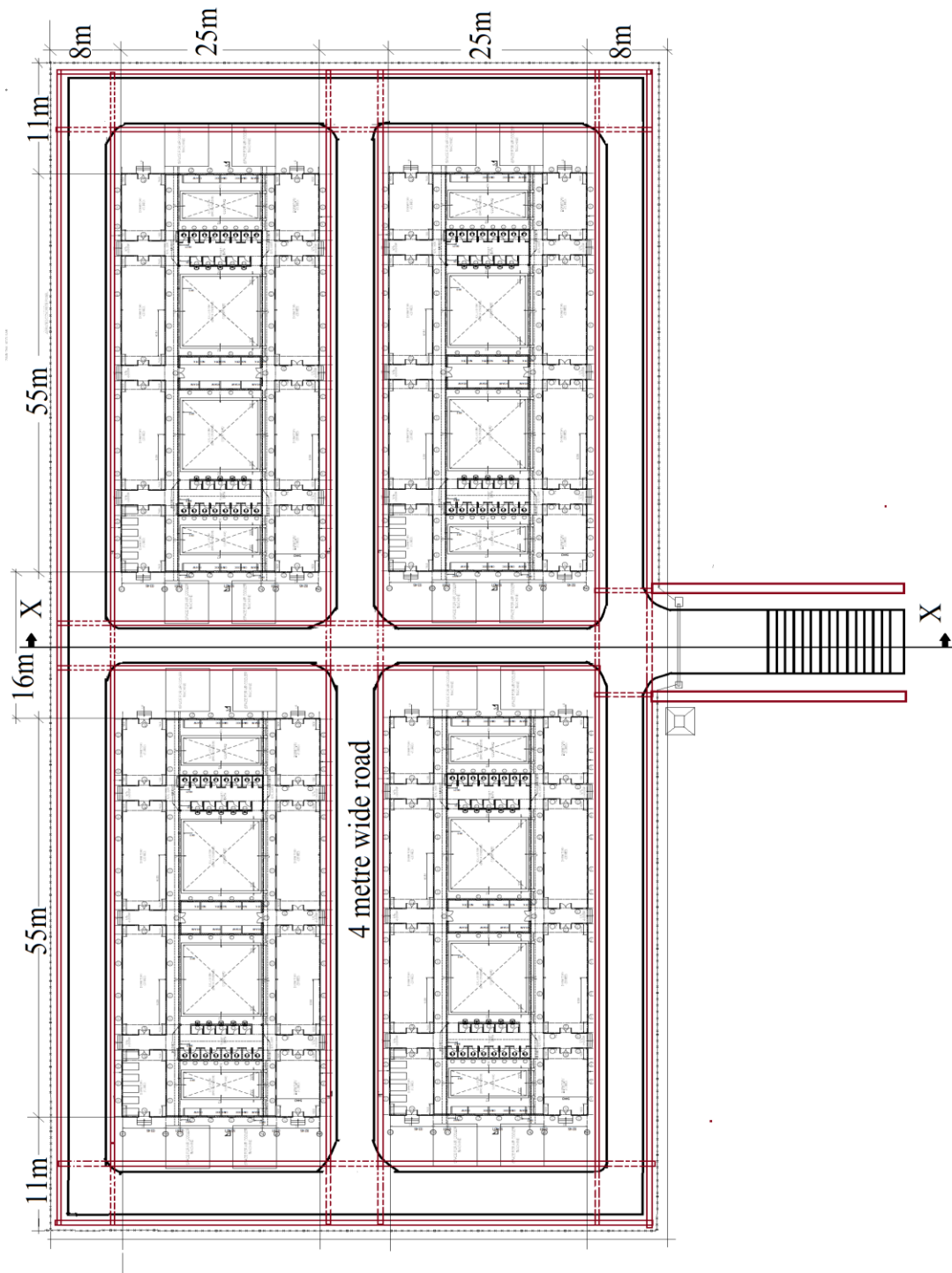
Drawing 2:- Labour/worker colony set up for 500 Workers.
