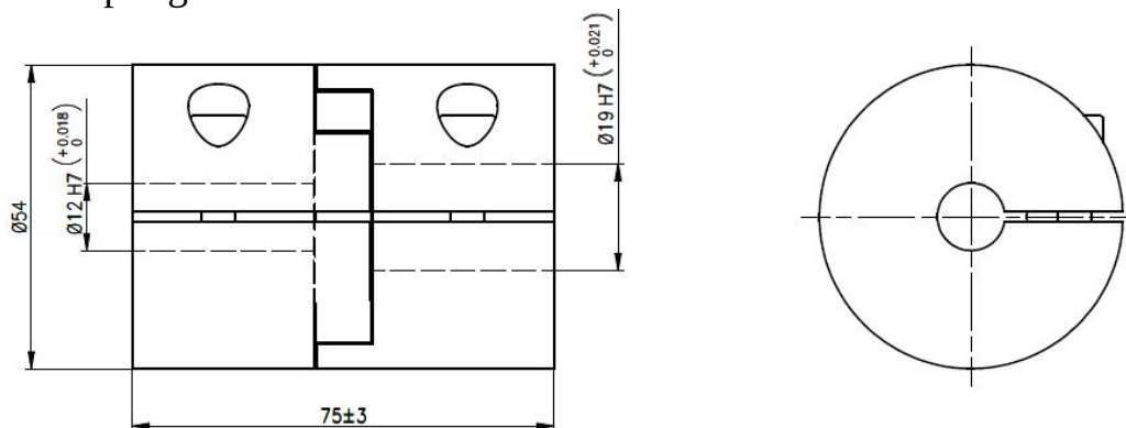
STAR COUPLING WITH SPLIT CLAMPING
