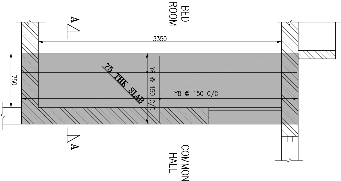
PLAN FOR LOFT REINF. (TYP.)
