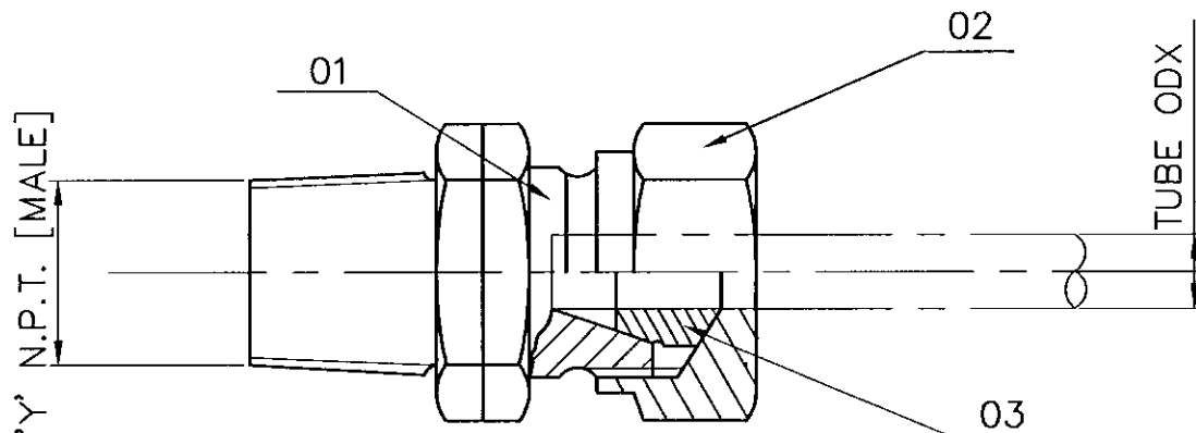
DETAIL OF FLARELESS 'BITE' TYPE FITTING
