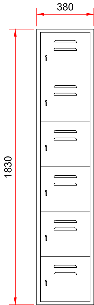
FRONT VIEW
