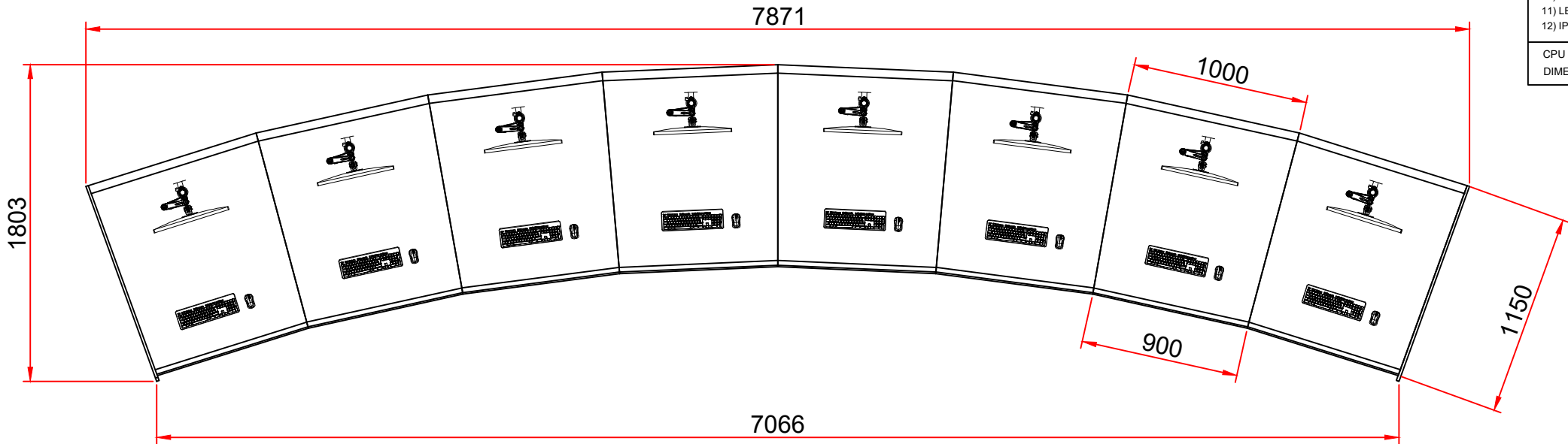
TOP VIEW
