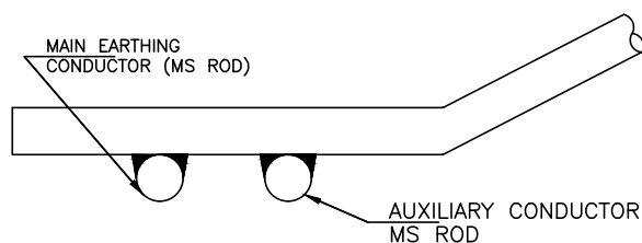
DETAIL-C
