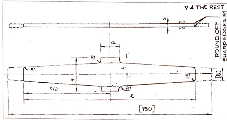
Fig.1. Flat Spring
