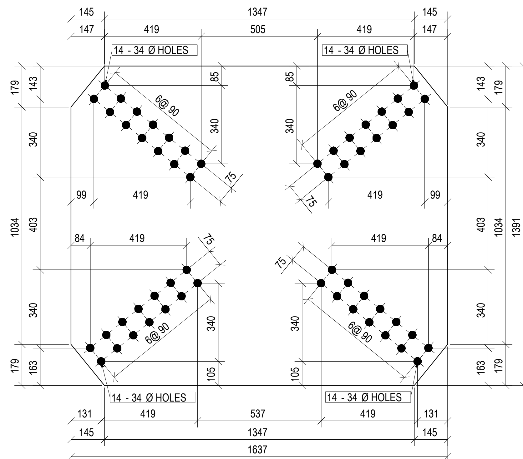
DETAIL OF ITEM NO. PLT-58
