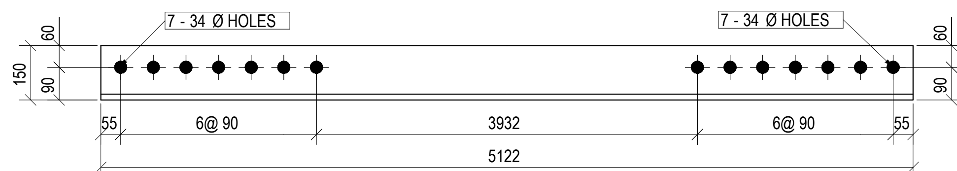
DETAIL OF ITEM NO. L-35
