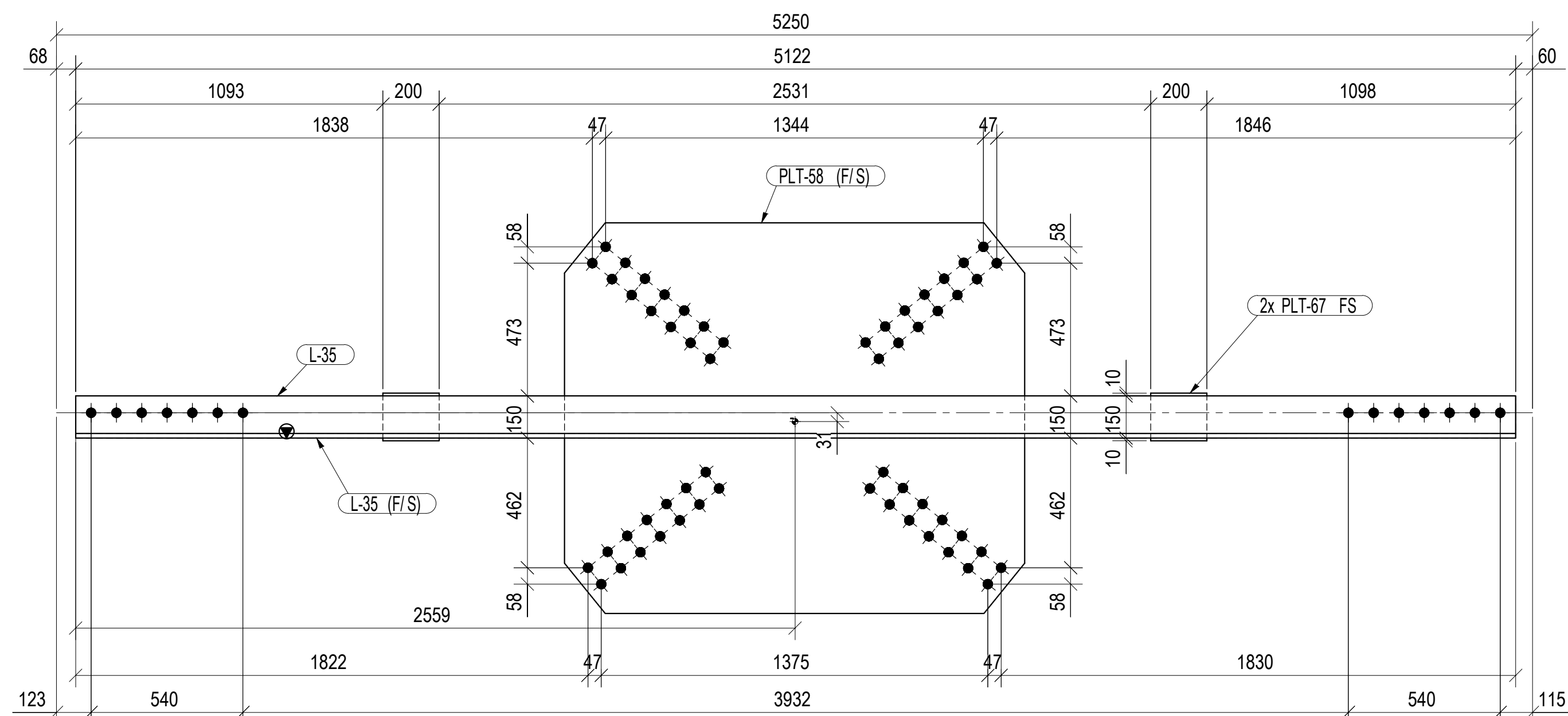
2-V-BRACEBS MARKED AS VBR260-136
