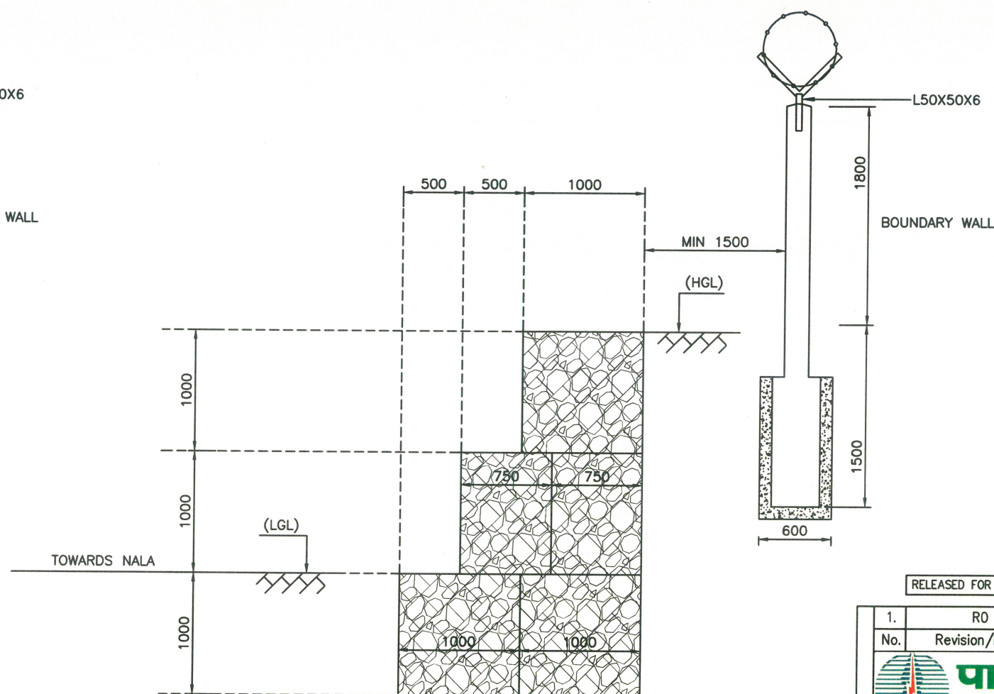
TYPICAL DETAILS OF 2 Mtr. GABION WALL
