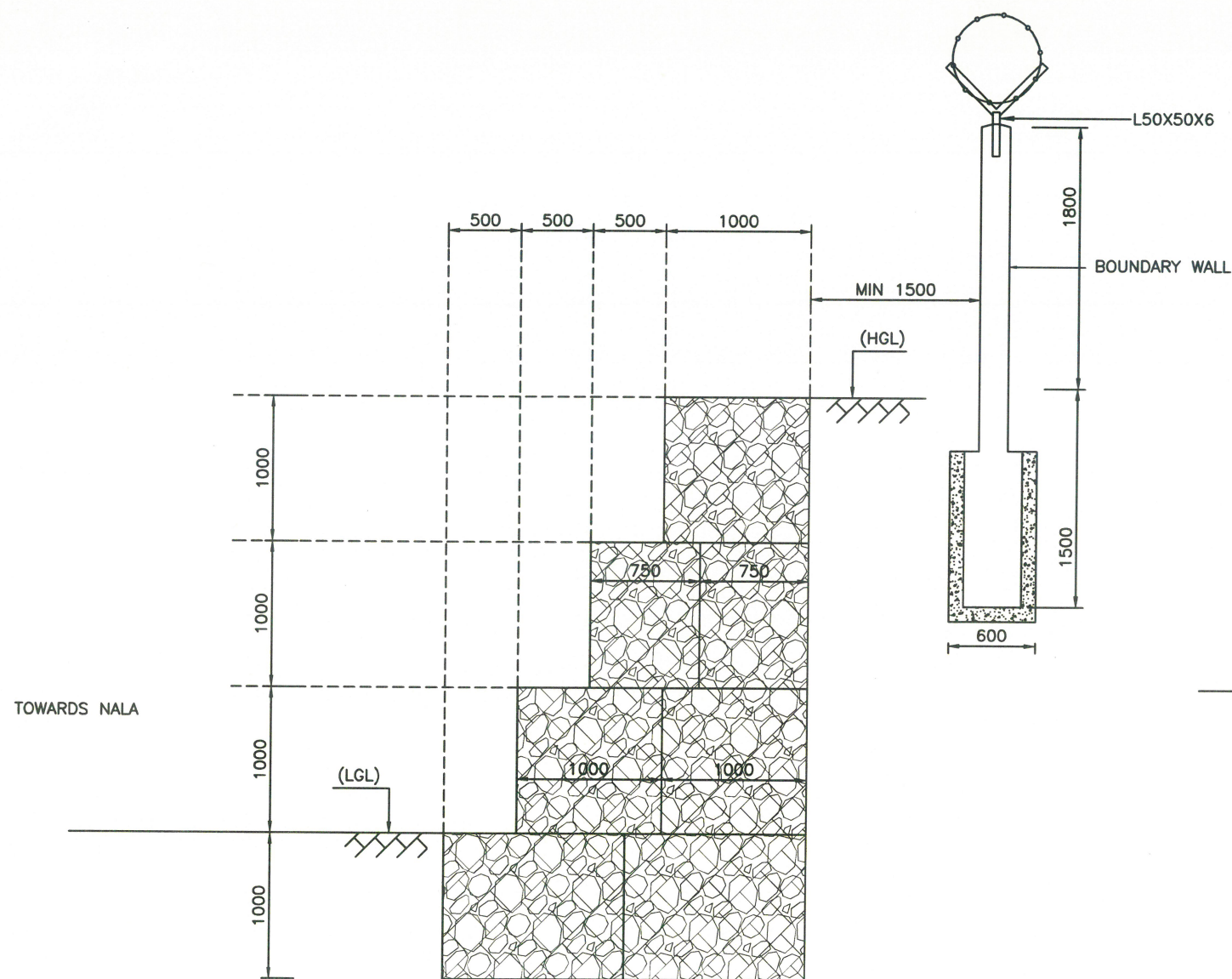
TYPICAL DETAILS OF 3 Mtr. GABION WALL
