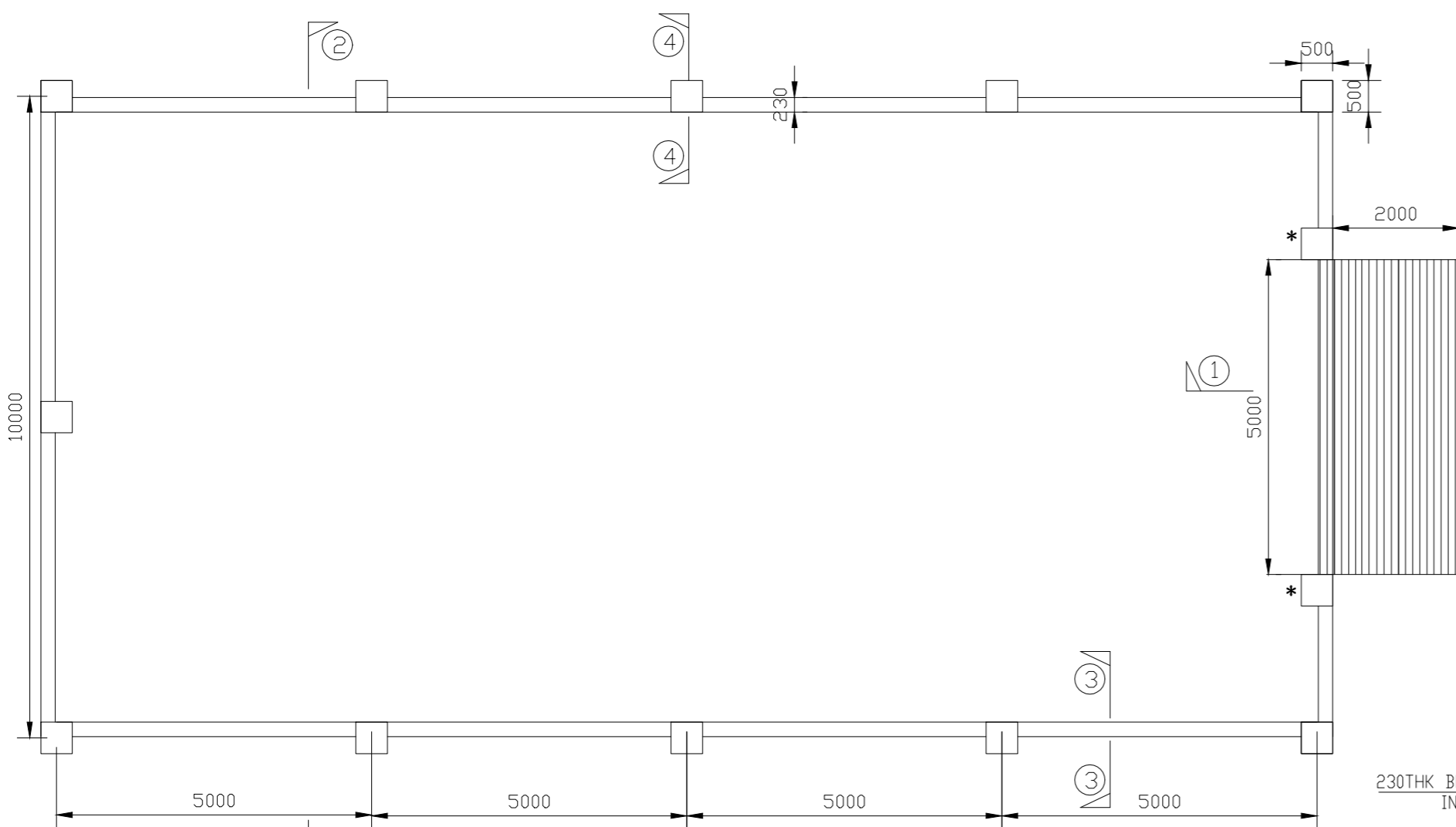
PLAN
