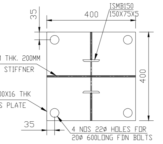
DETAIL OF BASE PLATE (TYP.)
