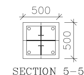
SECTION 5-5
