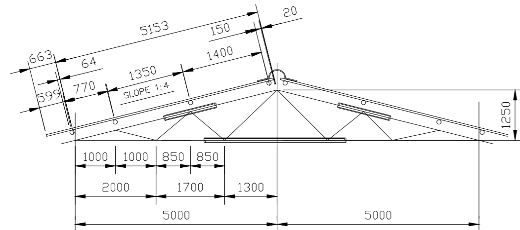
DETAIL OF TRUSS
