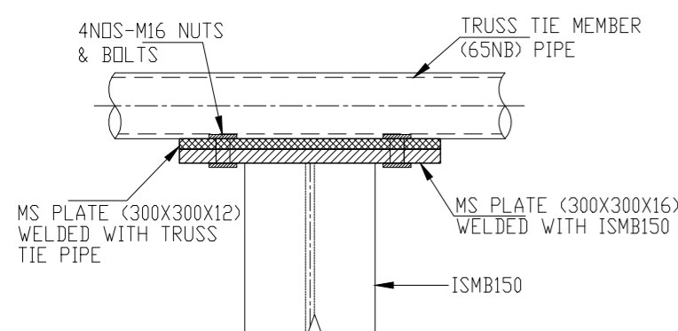
JOINT-1 (TYP.)
