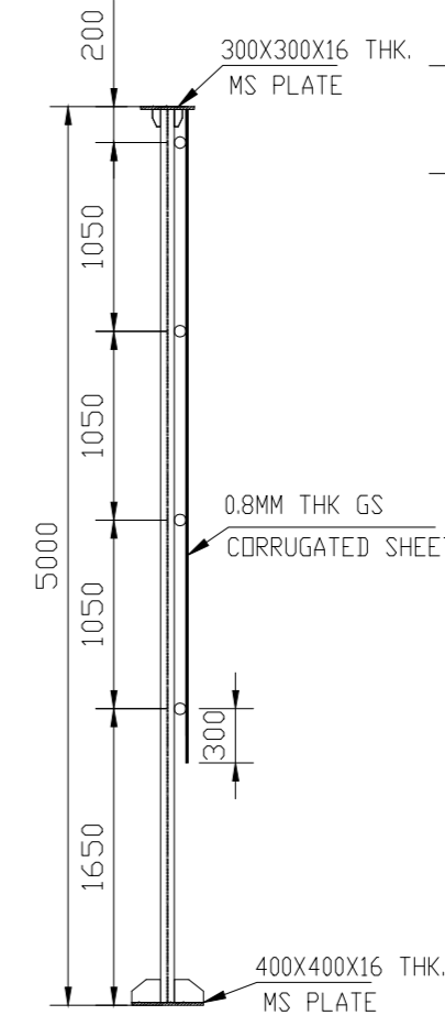
COLUMN & GIRT FIXING DETAILS (TYP.)
