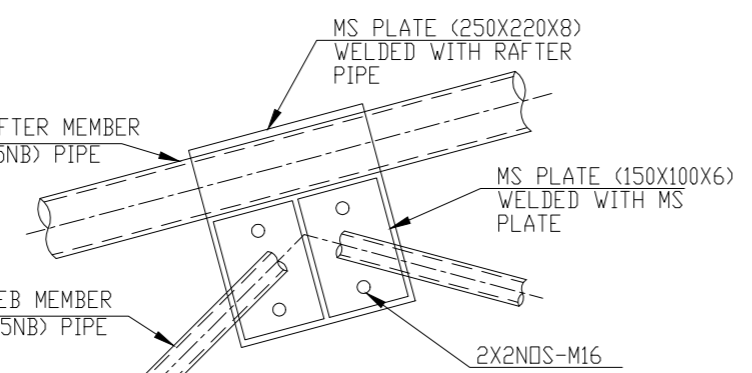
JOINT-5 (TYP.)
