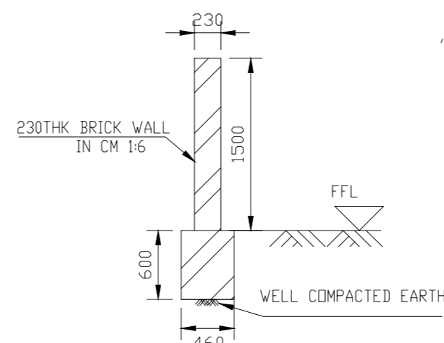
SECTION 3-3 (TYP.)
