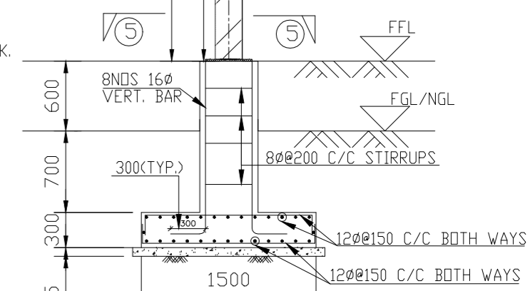
SECTION 4-4
