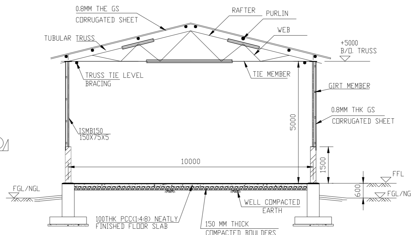
SECTION 2-2
