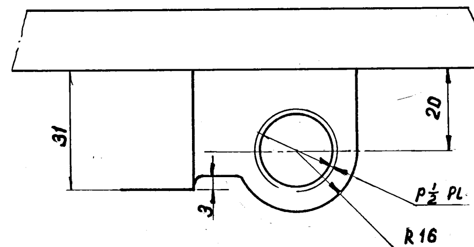
VIEW - A
