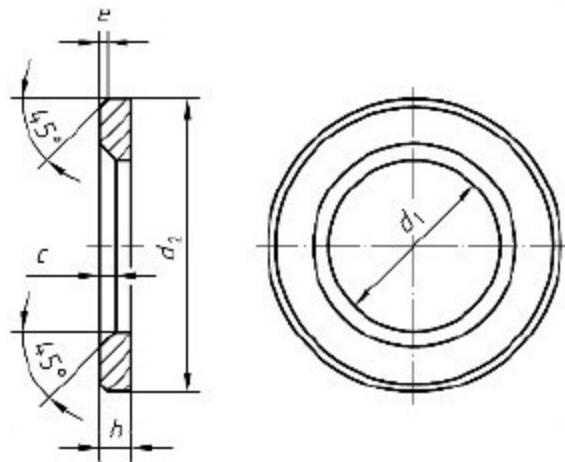
Figure 6 --- Dimensions
