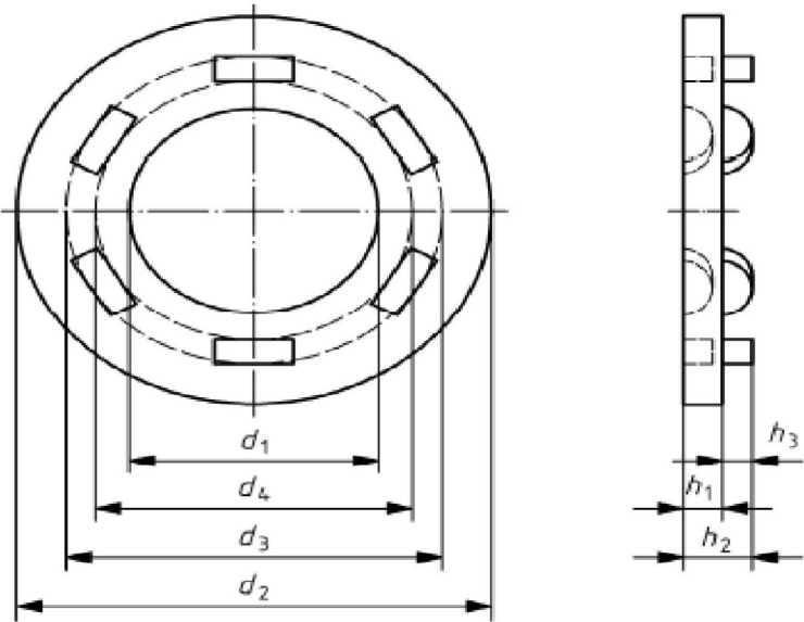
Figure 1 — Dimensions of compressible washer-type direct tension indicator (example with six protrusions)
