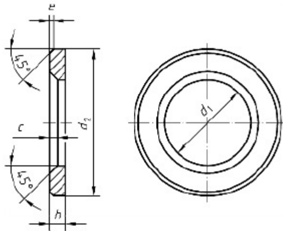
Figure 6 --- Dimensions
