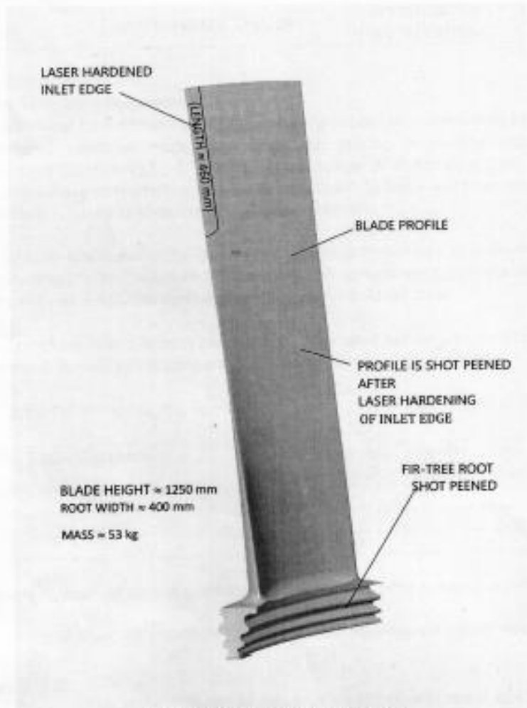
Figure 1: Blade details for reference
