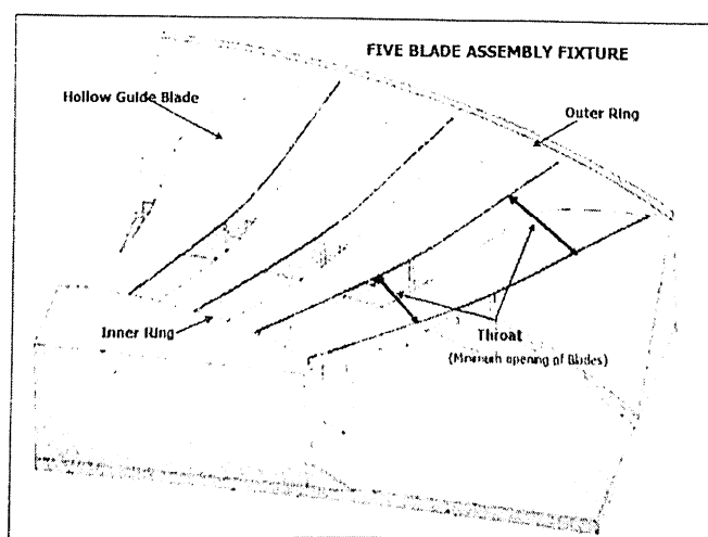
Figure. 2 (For Reference only. 5-Blade assembly fixture for 3L/3R Blade)
