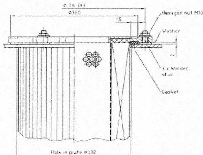
Clean side Installation of Filter Cartridges Ø 327 mm 3 lug flange (3 hooks)
