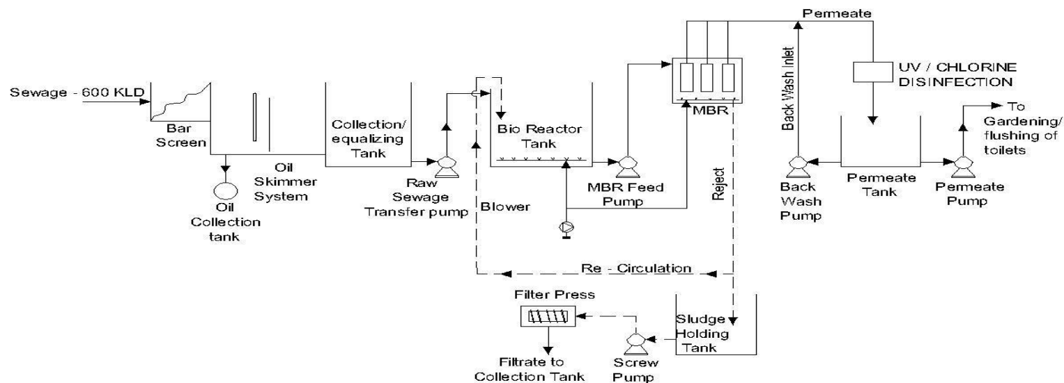
Indicative Process Flow Diagram
