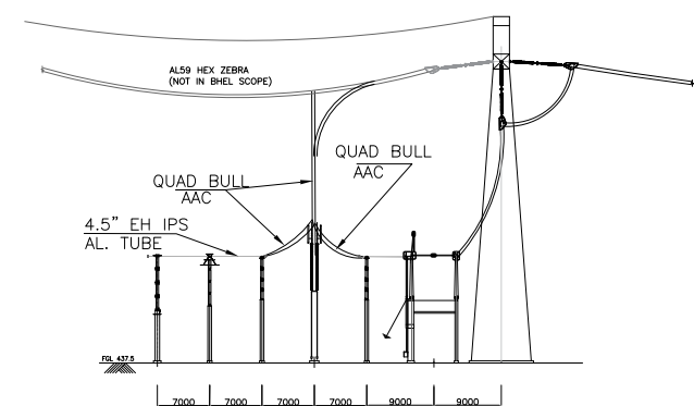
765KV LINE WITHOUT WAVE TRAP (TYPICAL SECTION)
