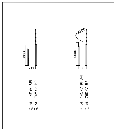
SECTION E-E
