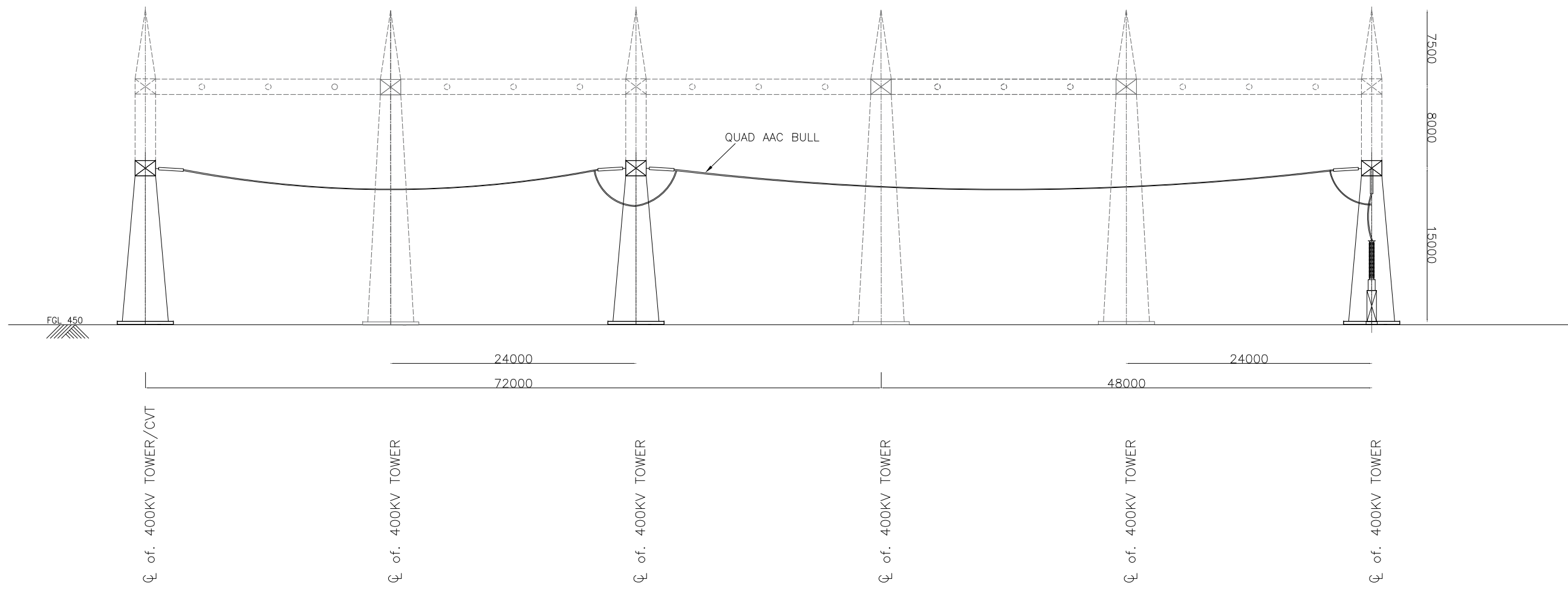
SECTION 4C-4C (400KV MAIN BUS-II)
