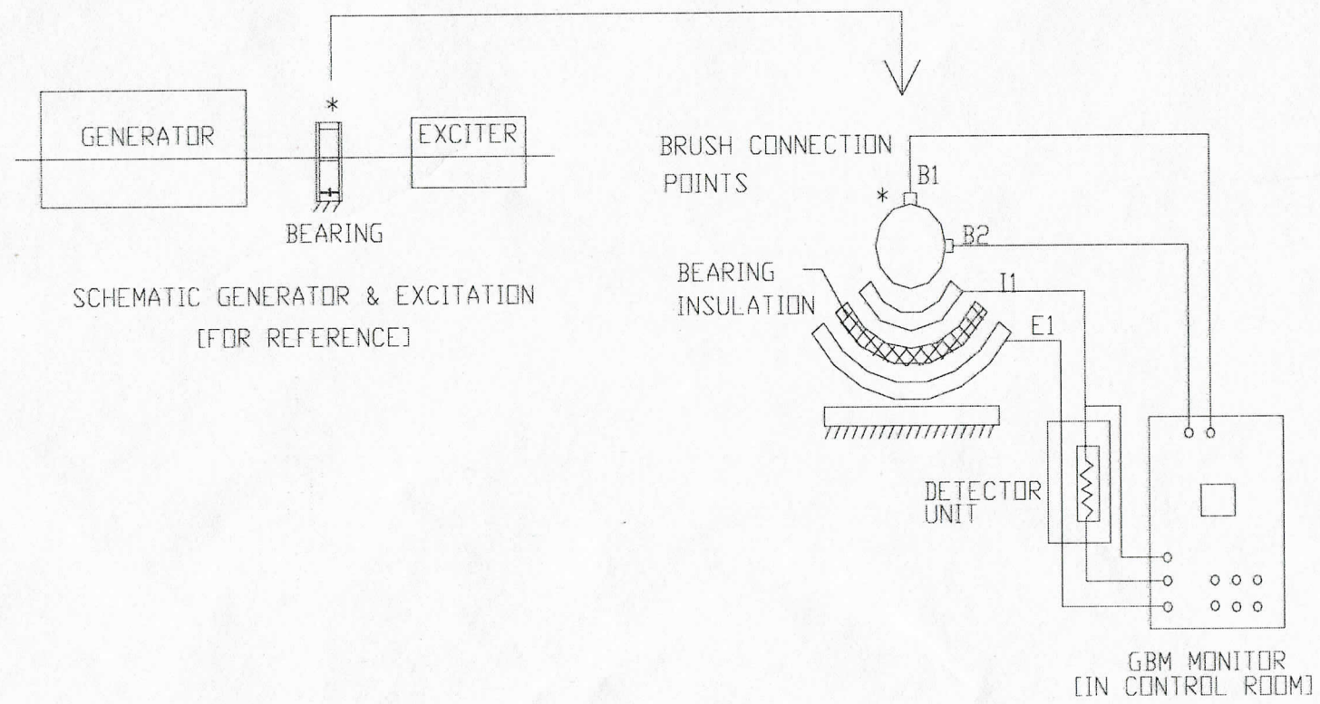
FIG: 1 SCHEMATIC OF TG SET AND SIGNAL TAPPING POINT FOR GBM (APPLICABLE FOR ALL TYPE OF GENERATORS)
