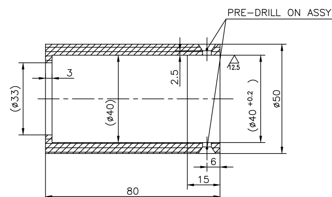
ITEM 2 MATERIAL: HP TUBE (INTERNAL DETAILS ARE FOR REFERENCE ONLY)
