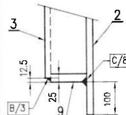
VIEW Y-Y
