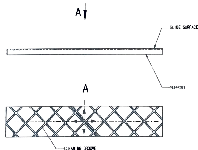
Schematic View of Lubricating Plates
