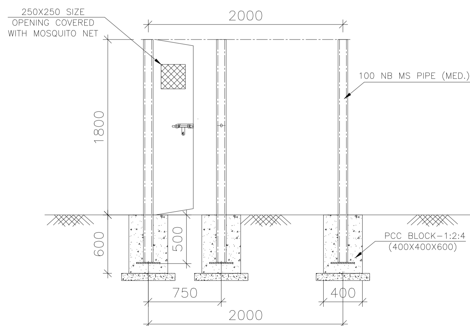
SECTION 3-3 (SCALE 1:1)
