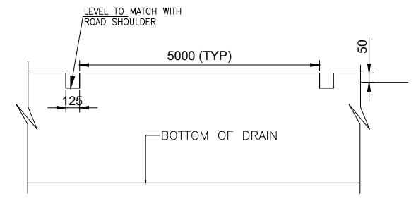
TYP. ELEVATION OF CUTOUT TOWARDS EARTHEN SIDE
