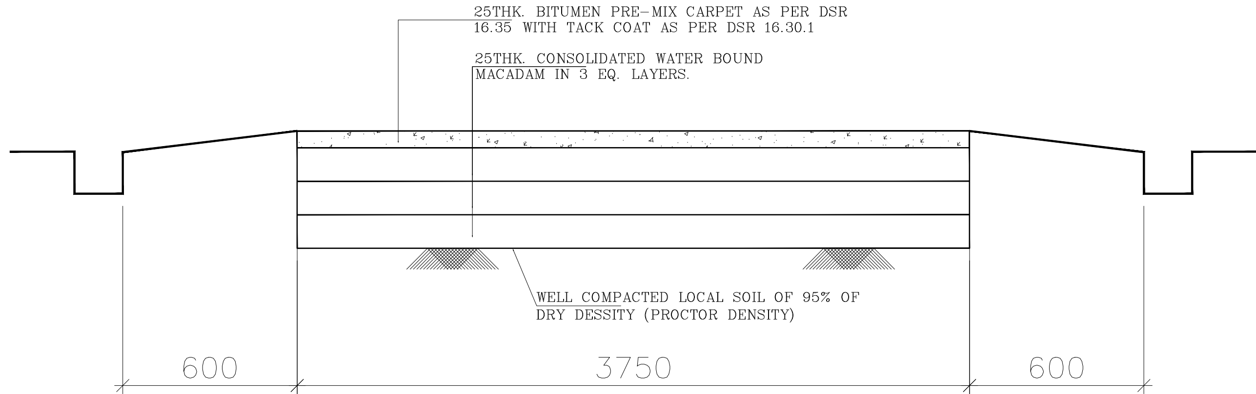
TYP CROSS SECTION OF 3.75M WIDE ROAD
