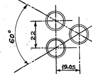
LAYOUT OF TUBE HOLES SCALE 1:1
