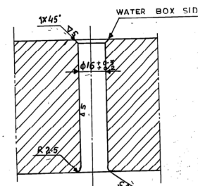
DRILLING DETAIL SCALE 1"=1'
