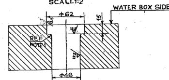
SECTION B-B SCALE 1:2
