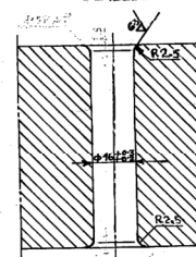
DRILLING DETAIL SCALE 1:1
