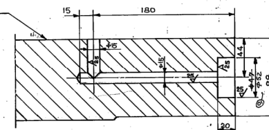
SECTION C-C SCALE 1:2
