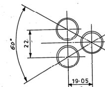
LAY OUT OF TUBE HOLES SCALE 1"=1
